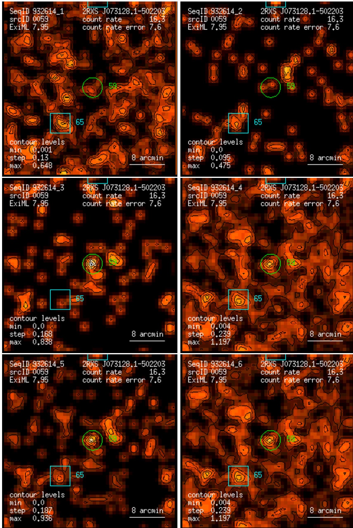
Figure 59: RASS 932614: detection 0059: band rate images, Gaussian filter: (1) PSPC channels 11 – 41, (2) 52 – 90, (3) 91 – 201, (4) 11 – 235, (5) 52 – 201, (6) 11 – 201. Broad band rates in counts/ks. Band rate contour levels in counts/ks/arcmin 2 .
