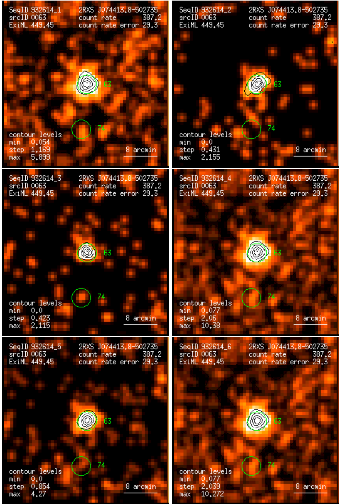
Figure 63: RASS 932614: detection 0063: band rate images, Gaussian filter: (1) PSPC channels 11 – 41, (2) 52 – 90, (3) 91 – 201, (4) 11 – 235, (5) 52 – 201, (6) 11 – 201. Broad band rates in counts/ks. Band rate contour levels in counts/ks/arcmin 2 .
