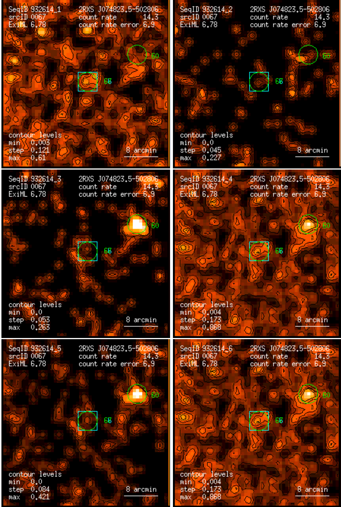
Figure 67: RASS 932614: detection 0067: band rate images, Gaussian filter: (1) PSPC channels 11 – 41, (2) 52 – 90, (3) 91 – 201, (4) 11 – 235, (5) 52 – 201, (6) 11 – 201. Broad band rates in counts/ks. Band rate contour levels in counts/ks/arcmin 2 .
