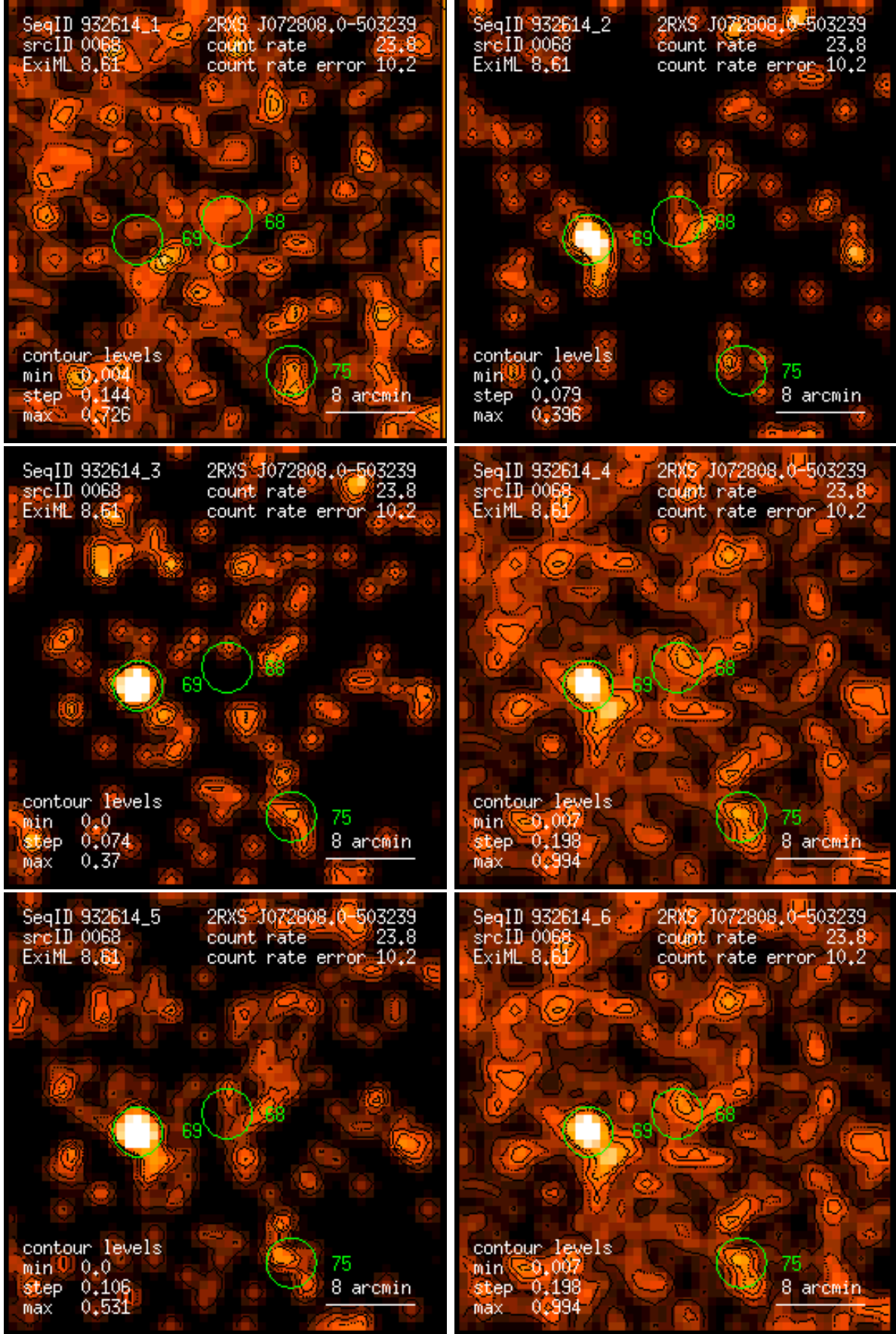
Figure 68: RASS 932614: detection 0068: band rate images, Gaussian filter: (1) PSPC channels 11 – 41, (2) 52 – 90, (3) 91 – 201, (4) 11 – 235, (5) 52 – 201, (6) 11 – 201. Broad band rates in counts/ks. Band rate contour levels in counts/ks/arcmin 2 .
