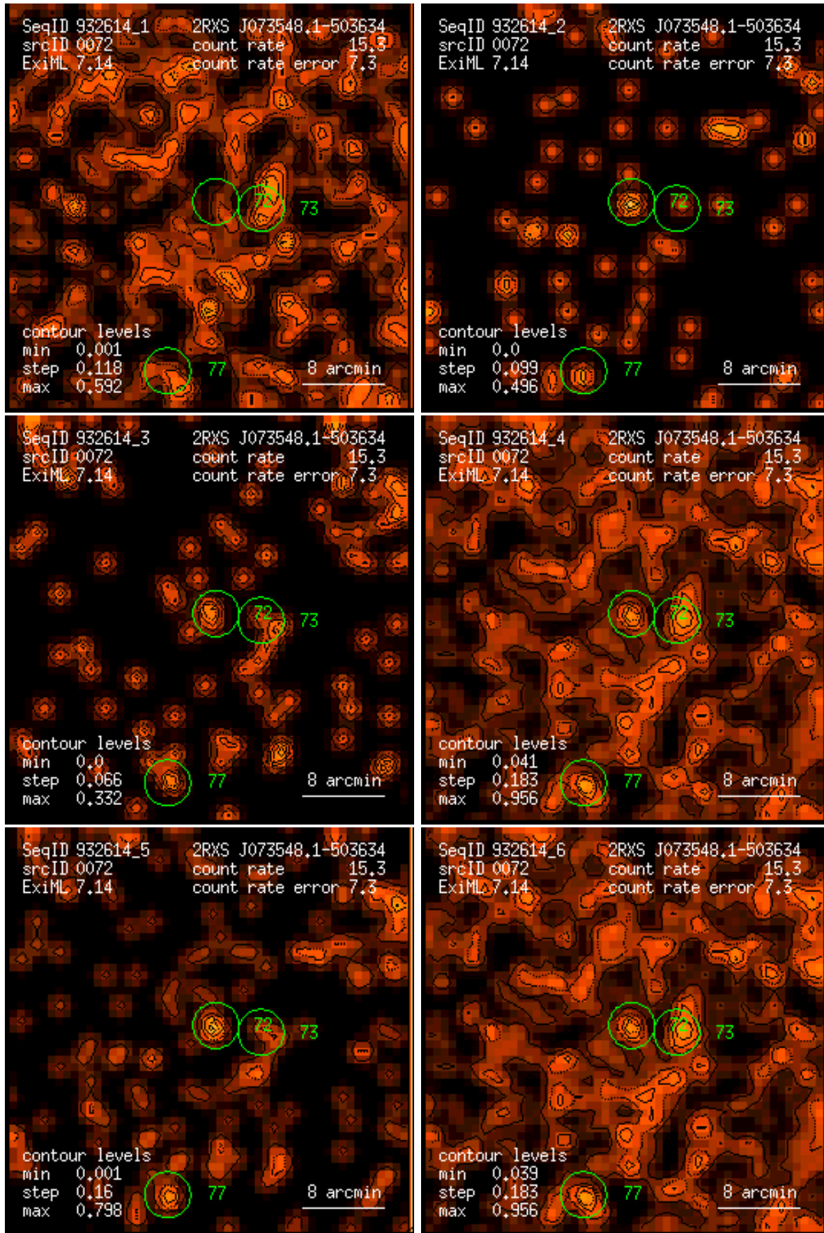
Figure 72: RASS 932614: detection 0072: band rate images, Gaussian filter: (1) PSPC channels 11 – 41, (2) 52 – 90, (3) 91 – 201, (4) 11 – 235, (5) 52 – 201, (6) 11 – 201. Broad band rates in counts/ks. Band rate contour levels in counts/ks/arcmin 2 .
