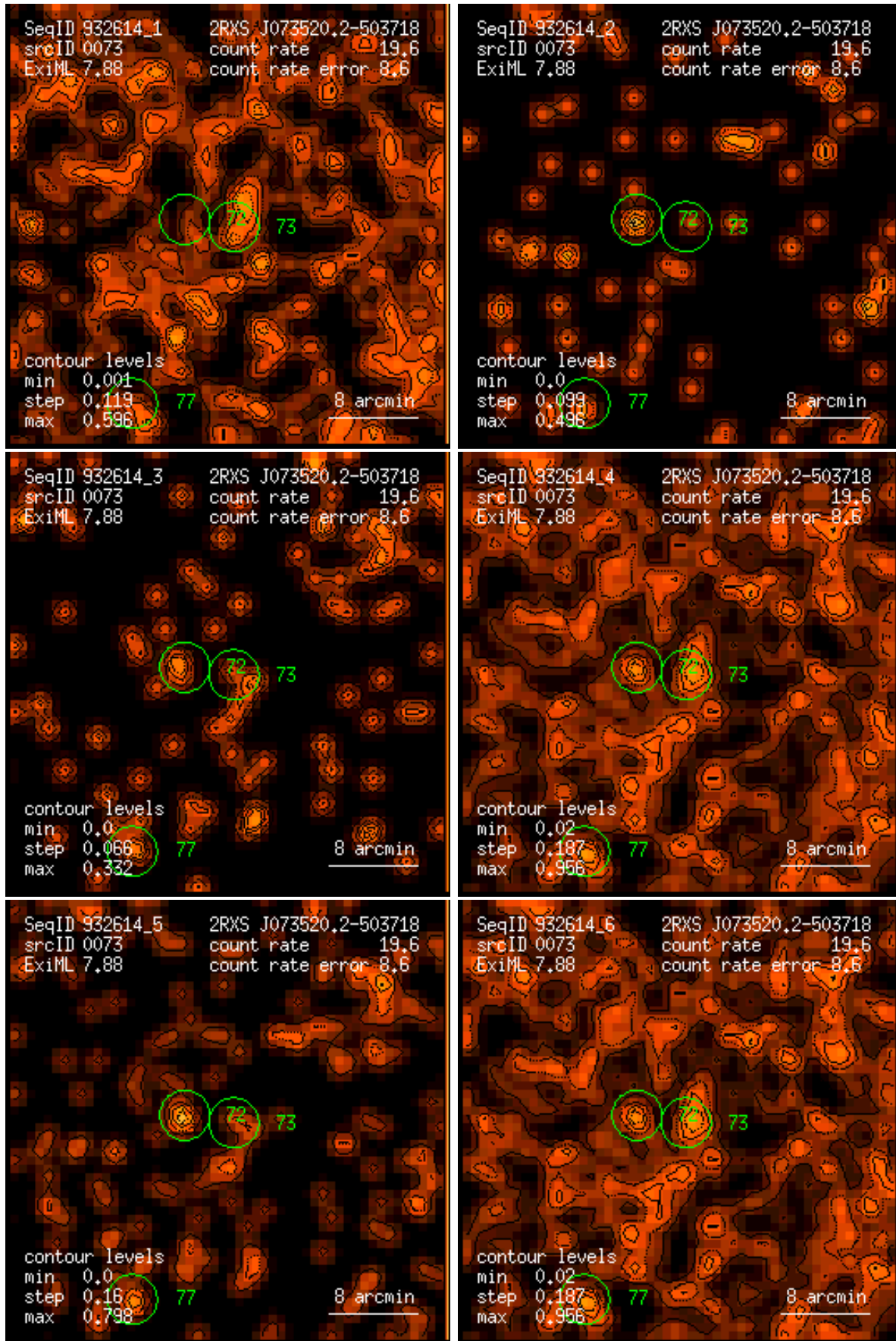
Figure 73: RASS 932614: detection 0073: band rate images, Gaussian filter: (1) PSPC channels 11 – 41, (2) 52 – 90, (3) 91 – 201, (4) 11 – 235, (5) 52 – 201, (6) 11 – 201. Broad band rates in counts/ks. Band rate contour levels in counts/ks/arcmin 2 .
