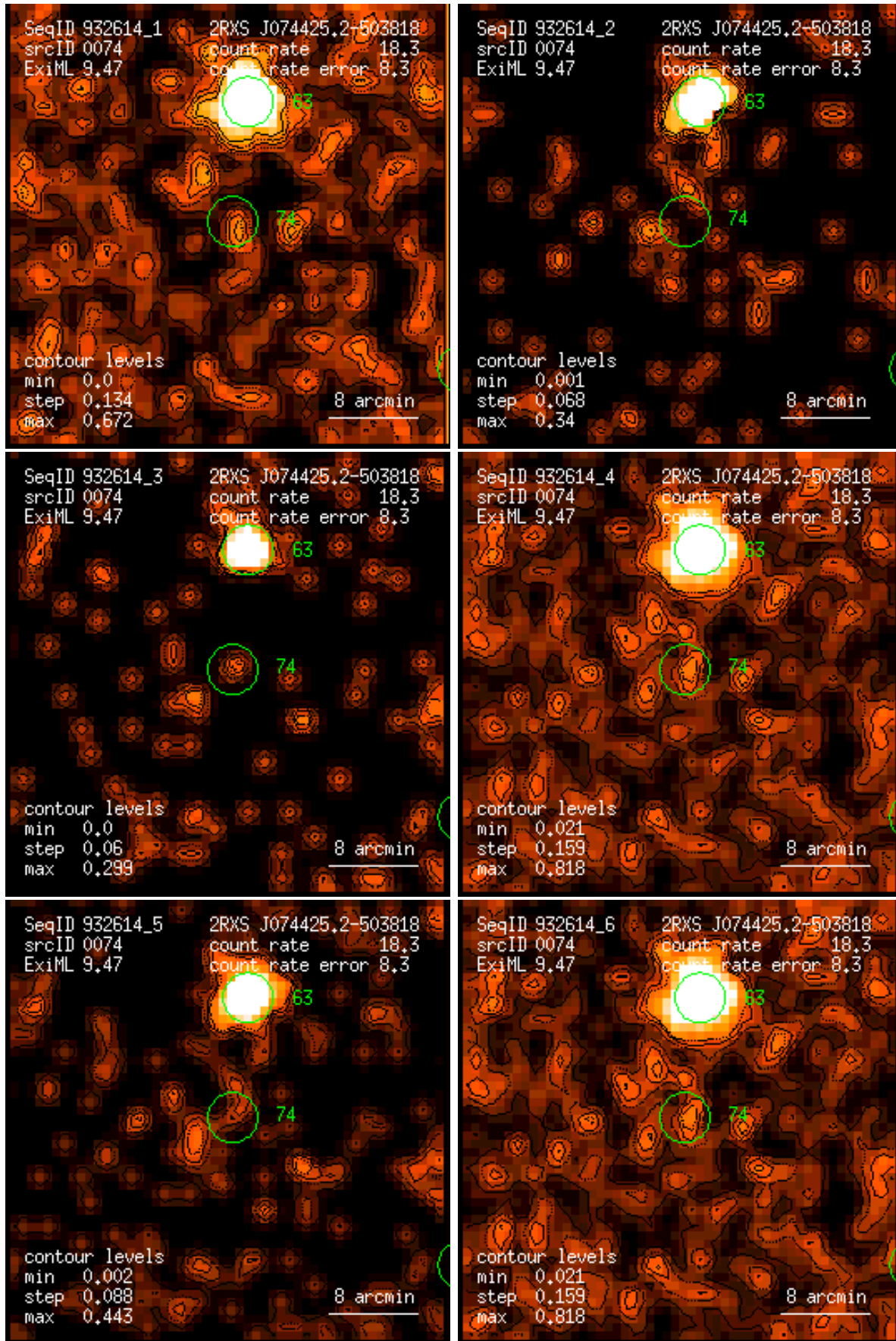
Figure 74: RASS 932614: detection 0074: band rate images, Gaussian filter: (1) PSPC channels 11 – 41, (2) 52 – 90, (3) 91 – 201, (4) 11 – 235, (5) 52 – 201, (6) 11 – 201. Broad band rates in counts/ks. Band rate contour levels in counts/ks/arcmin 2 .
