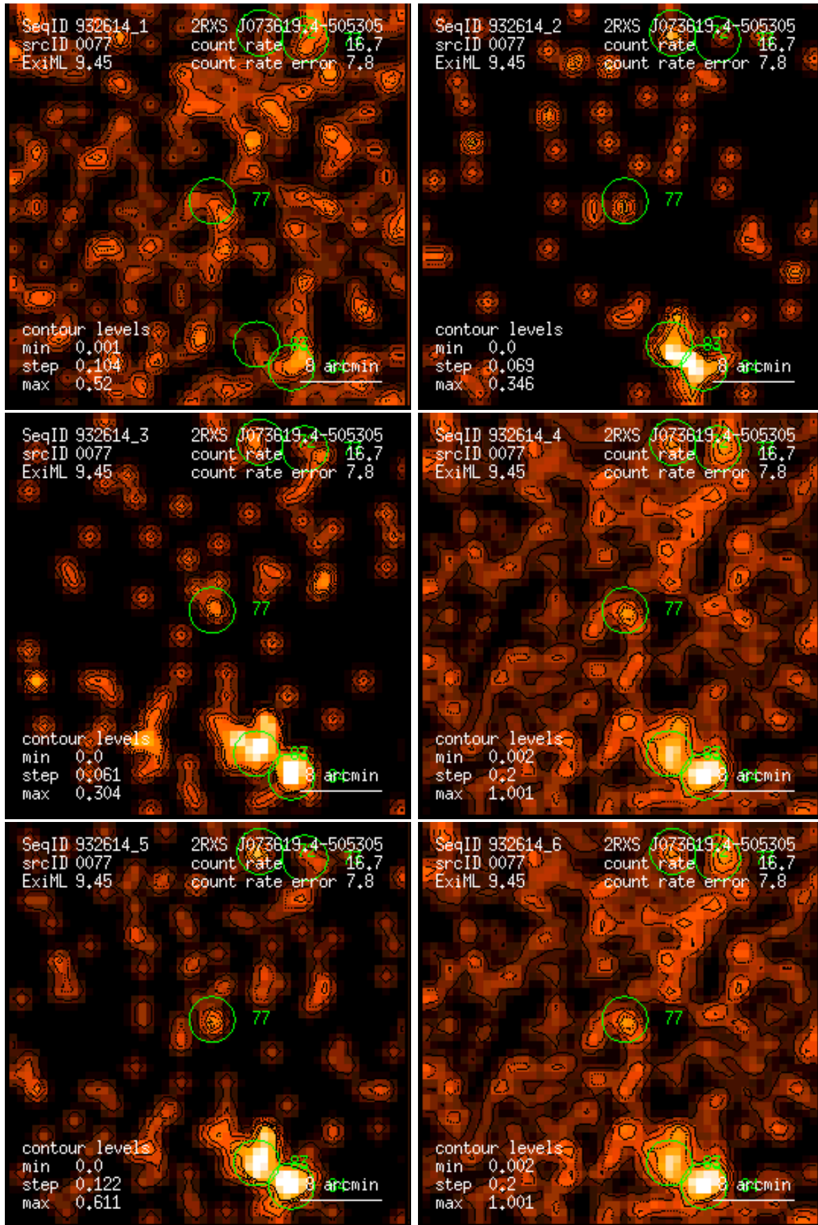
Figure 77: RASS 932614: detection 0077: band rate images, Gaussian filter: (1) PSPC channels 11 – 41, (2) 52 – 90, (3) 91 – 201, (4) 11 – 235, (5) 52 – 201, (6) 11 – 201. Broad band rates in counts/ks. Band rate contour levels in counts/ks/arcmin 2 .
