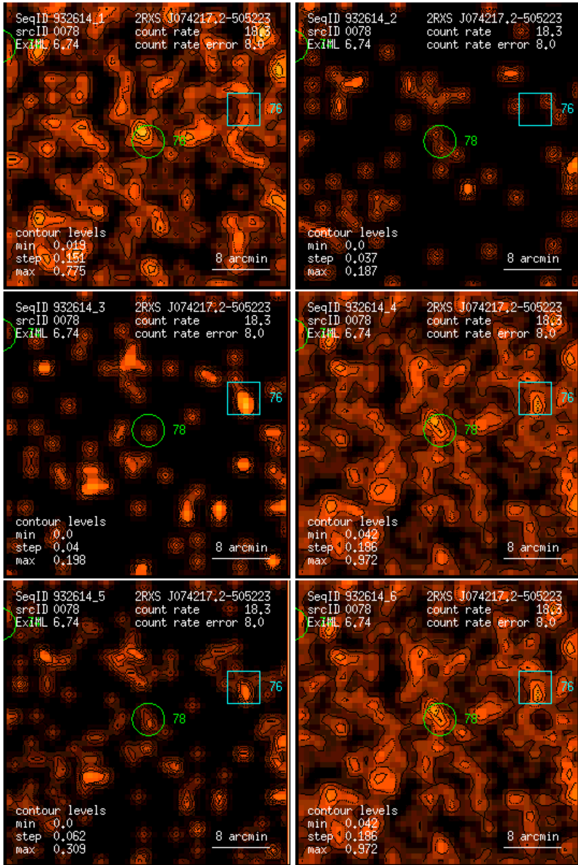
Figure 78: RASS 932614: detection 0078: band rate images, Gaussian filter: (1) PSPC channels 11 – 41, (2) 52 – 90, (3) 91 – 201, (4) 11 – 235, (5) 52 – 201, (6) 11 – 201. Broad band rates in counts/ks. Band rate contour levels in counts/ks/arcmin 2 .
