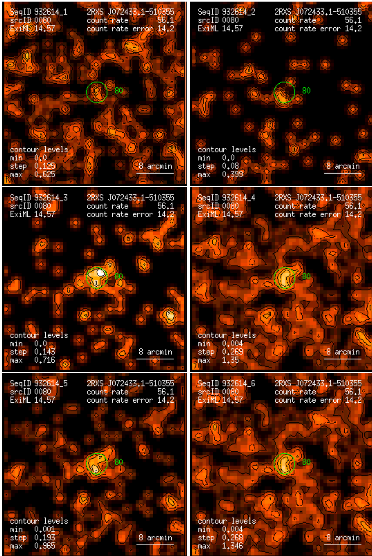
Figure 80: RASS 932614: detection 0080: band rate images, Gaussian filter: (1) PSPC channels 11 – 41, (2) 52 – 90, (3) 91 – 201, (4) 11 – 235, (5) 52 – 201, (6) 11 – 201. Broad band rates in counts/ks. Band rate contour levels in counts/ks/arcmin 2 .
