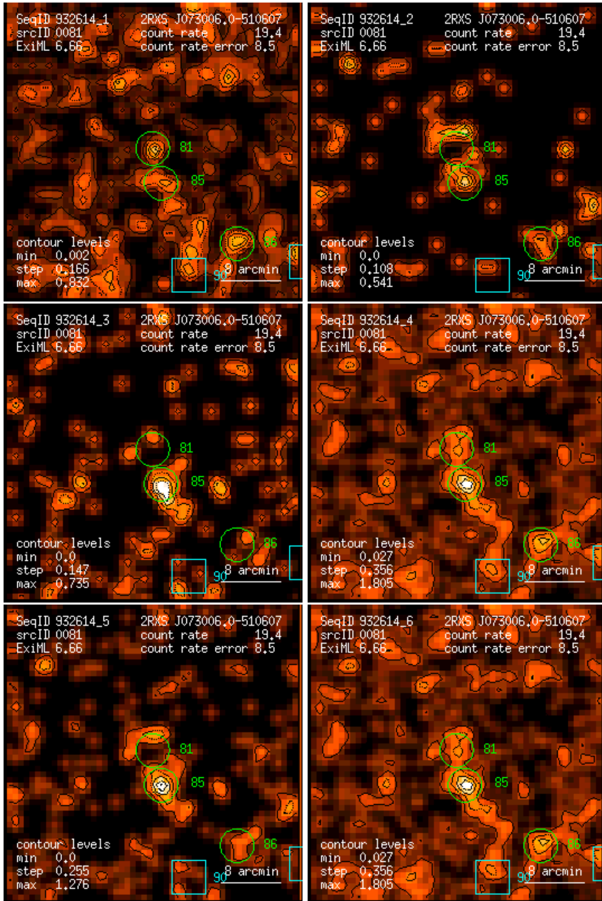
Figure 81: RASS 932614: detection 0081: band rate images, Gaussian filter: (1) PSPC channels 11 – 41, (2) 52 – 90, (3) 91 – 201, (4) 11 – 235, (5) 52 – 201, (6) 11 – 201. Broad band rates in counts/ks. Band rate contour levels in counts/ks/arcmin 2 .
