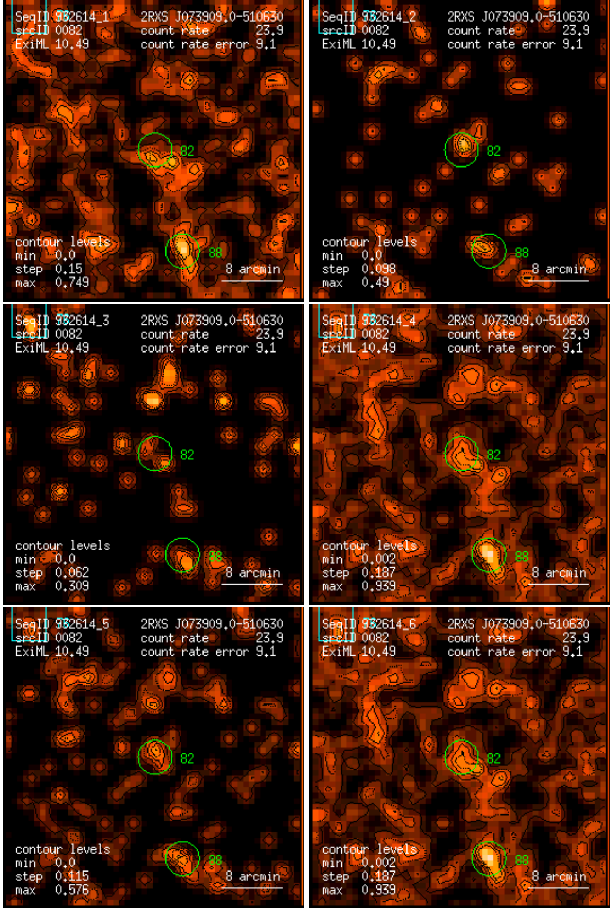
Figure 82: RASS 932614: detection 0082: band rate images, Gaussian filter: (1) PSPC channels 11 – 41, (2) 52 – 90, (3) 91 – 201, (4) 11 – 235, (5) 52 – 201, (6) 11 – 201. Broad band rates in counts/ks. Band rate contour levels in counts/ks/arcmin 2 .
