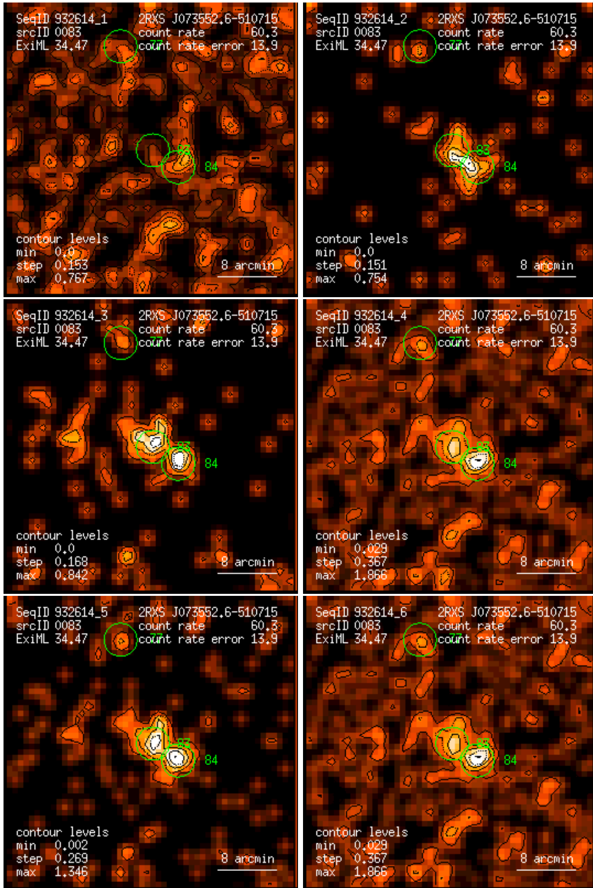
Figure 83: RASS 932614: detection 0083: band rate images, Gaussian filter: (1) PSPC channels 11 – 41, (2) 52 – 90, (3) 91 – 201, (4) 11 – 235, (5) 52 – 201, (6) 11 – 201. Broad band rates in counts/ks. Band rate contour levels in counts/ks/arcmin 2 .
