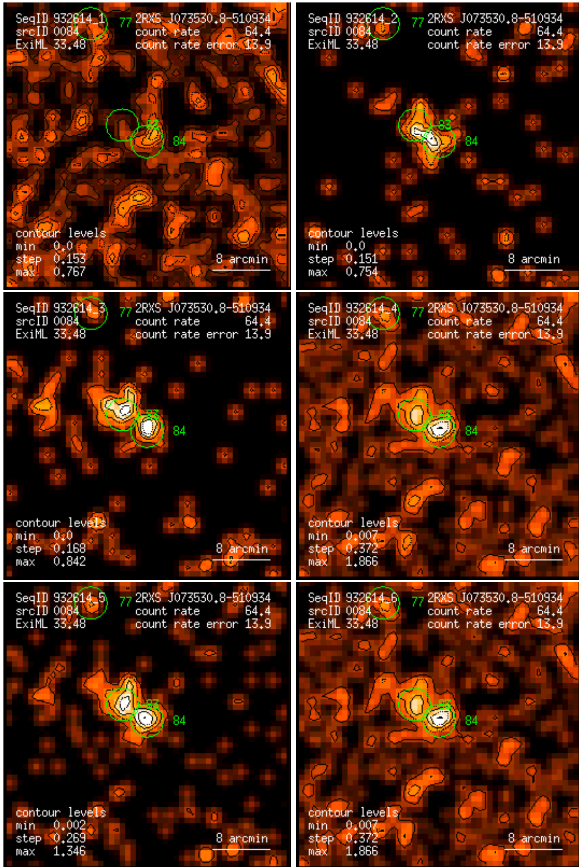
Figure 84: RASS 932614: detection 0084: band rate images, Gaussian filter: (1) PSPC channels 11 – 41, (2) 52 – 90, (3) 91 – 201, (4) 11 – 235, (5) 52 – 201, (6) 11 – 201. Broad band rates in counts/ks. Band rate contour levels in counts/ks/arcmin 2 .
