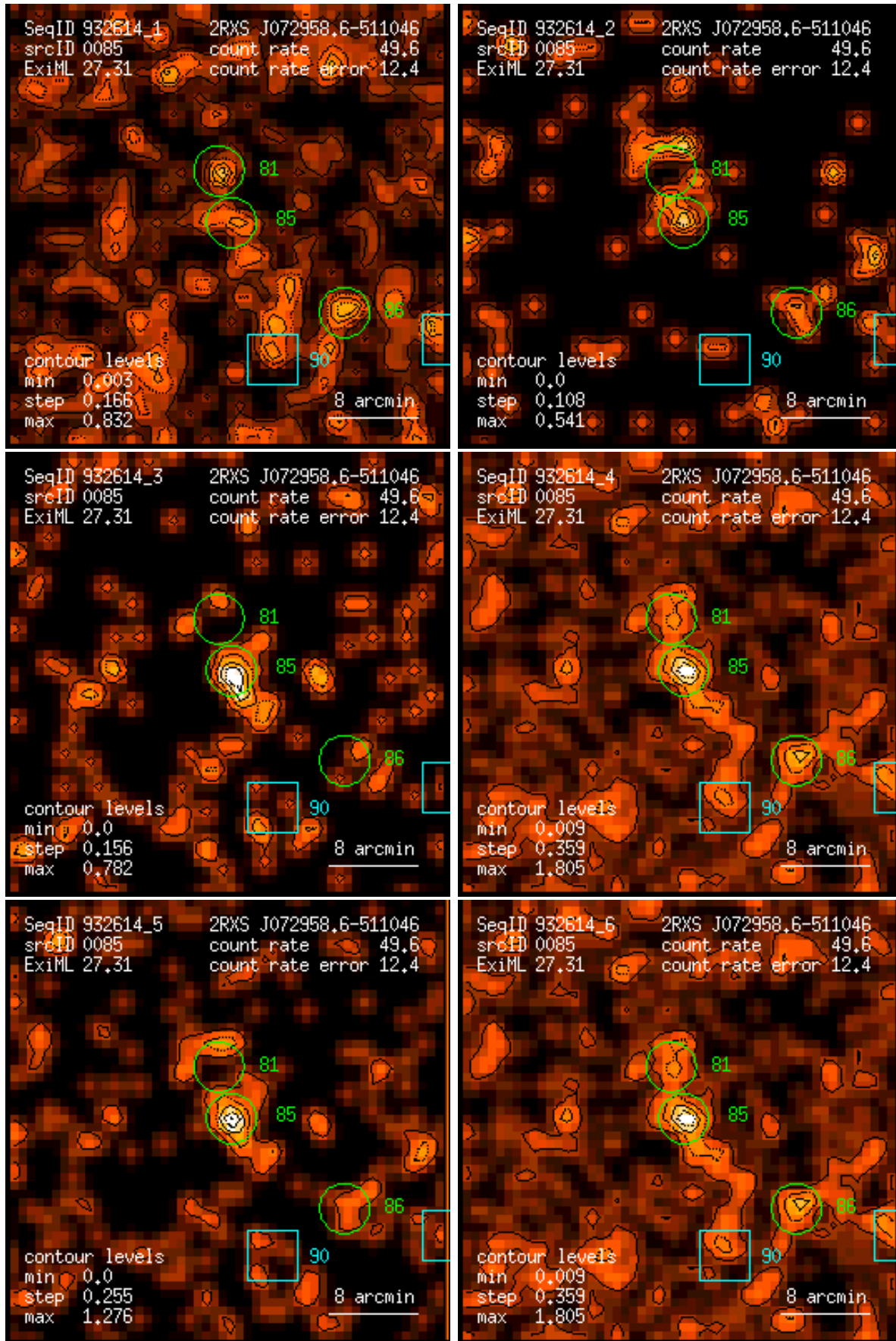
Figure 85: RASS 932614: detection 0085: band rate images, Gaussian filter: (1) PSPC channels 11 – 41, (2) 52 – 90, (3) 91 – 201, (4) 11 – 235, (5) 52 – 201, (6) 11 – 201. Broad band rates in counts/ks. Band rate contour levels in counts/ks/arcmin 2 .
