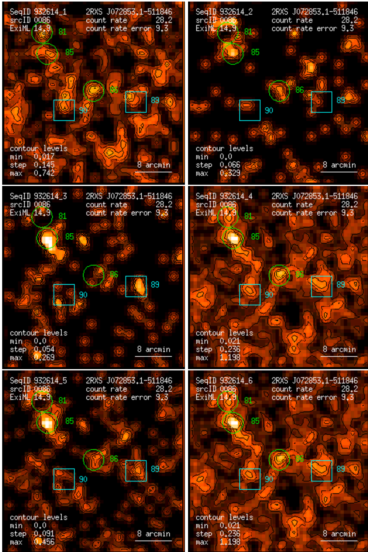
Figure 86: RASS 932614: detection 0086: band rate images, Gaussian filter: (1) PSPC channels 11 – 41, (2) 52 – 90, (3) 91 – 201, (4) 11 – 235, (5) 52 – 201, (6) 11 – 201. Broad band rates in counts/ks. Band rate contour levels in counts/ks/arcmin 2 .
