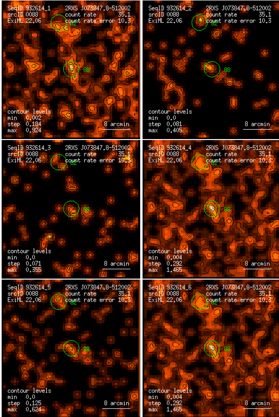
Figure 88: RASS 932614: detection 0088: band rate images, Gaussian filter: (1) PSPC channels 11 – 41, (2) 52 – 90, (3) 91 – 201, (4) 11 – 235, (5) 52 – 201, (6) 11 – 201. Broad band rates in counts/ks. Band rate contour levels in counts/ks/arcmin 2 .
