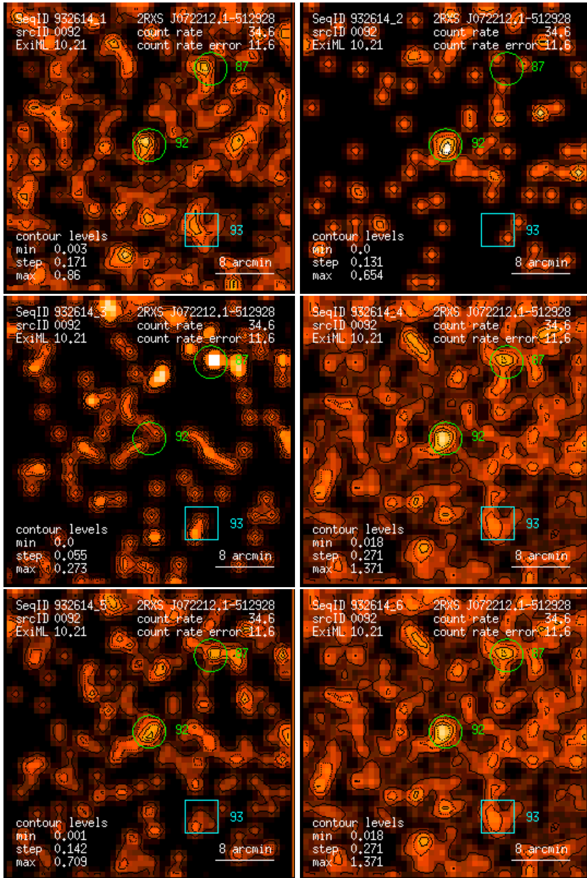
Figure 92: RASS 932614: detection 0092: band rate images, Gaussian filter: (1) PSPC channels 11 – 41, (2) 52 – 90, (3) 91 – 201, (4) 11 – 235, (5) 52 – 201, (6) 11 – 201. Broad band rates in counts/ks. Band rate contour levels in counts/ks/arcmin 2 .
