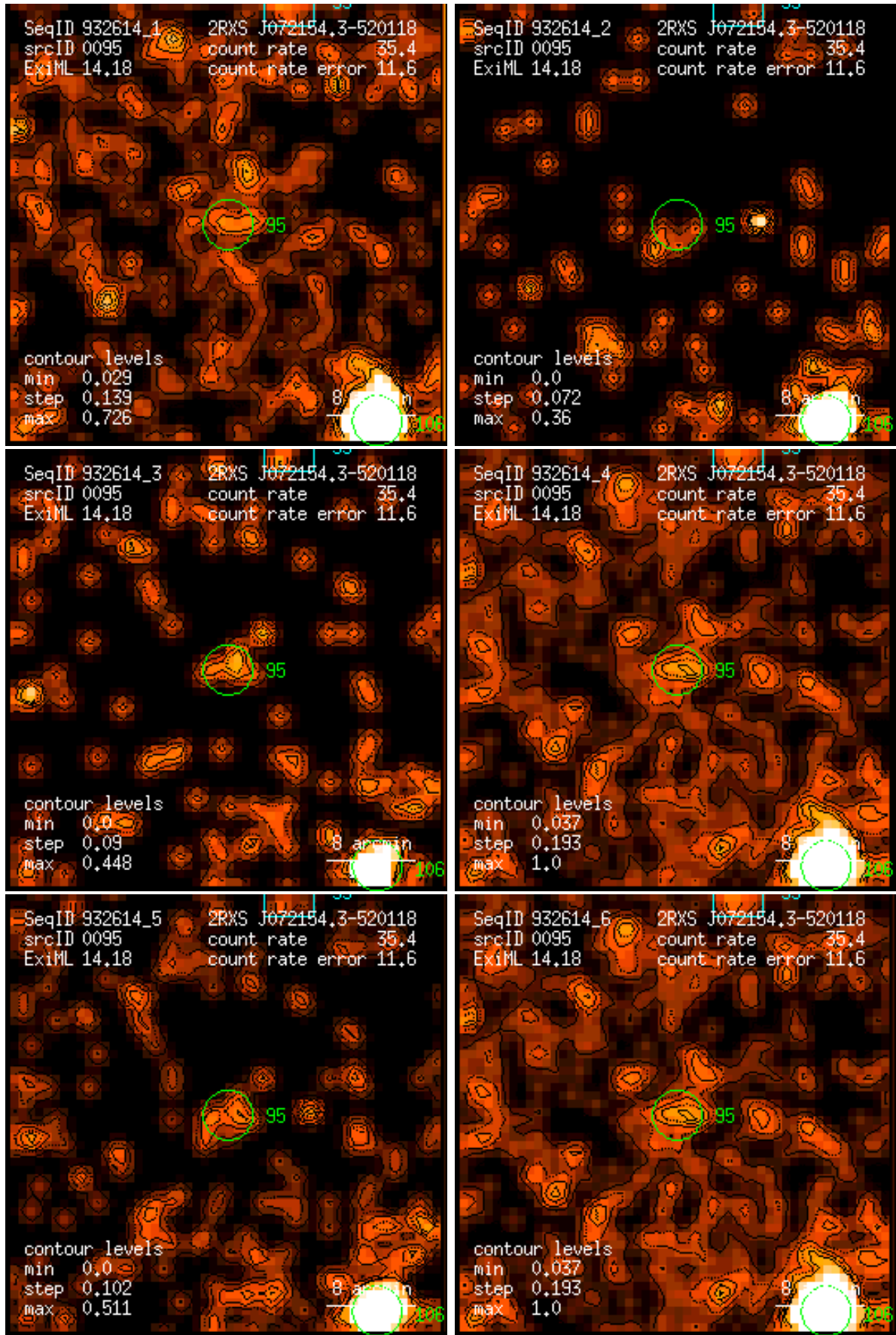
Figure 95: RASS 932614: detection 0095: band rate images, Gaussian filter: (1) PSPC channels 11 – 41, (2) 52 – 90, (3) 91 – 201, (4) 11 – 235, (5) 52 – 201, (6) 11 – 201. Broad band rates in counts/ks. Band rate contour levels in counts/ks/arcmin 2 .
