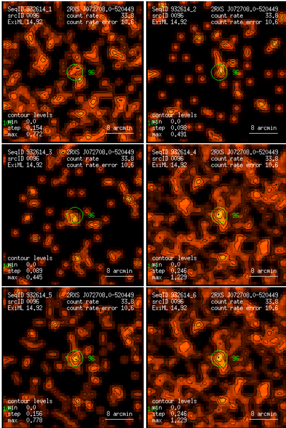
Figure 96: RASS 932614: detection 0096: band rate images, Gaussian filter: (1) PSPC channels 11 – 41, (2) 52 – 90, (3) 91 – 201, (4) 11 – 235, (5) 52 – 201, (6) 11 – 201. Broad band rates in counts/ks. Band rate contour levels in counts/ks/arcmin 2 .
