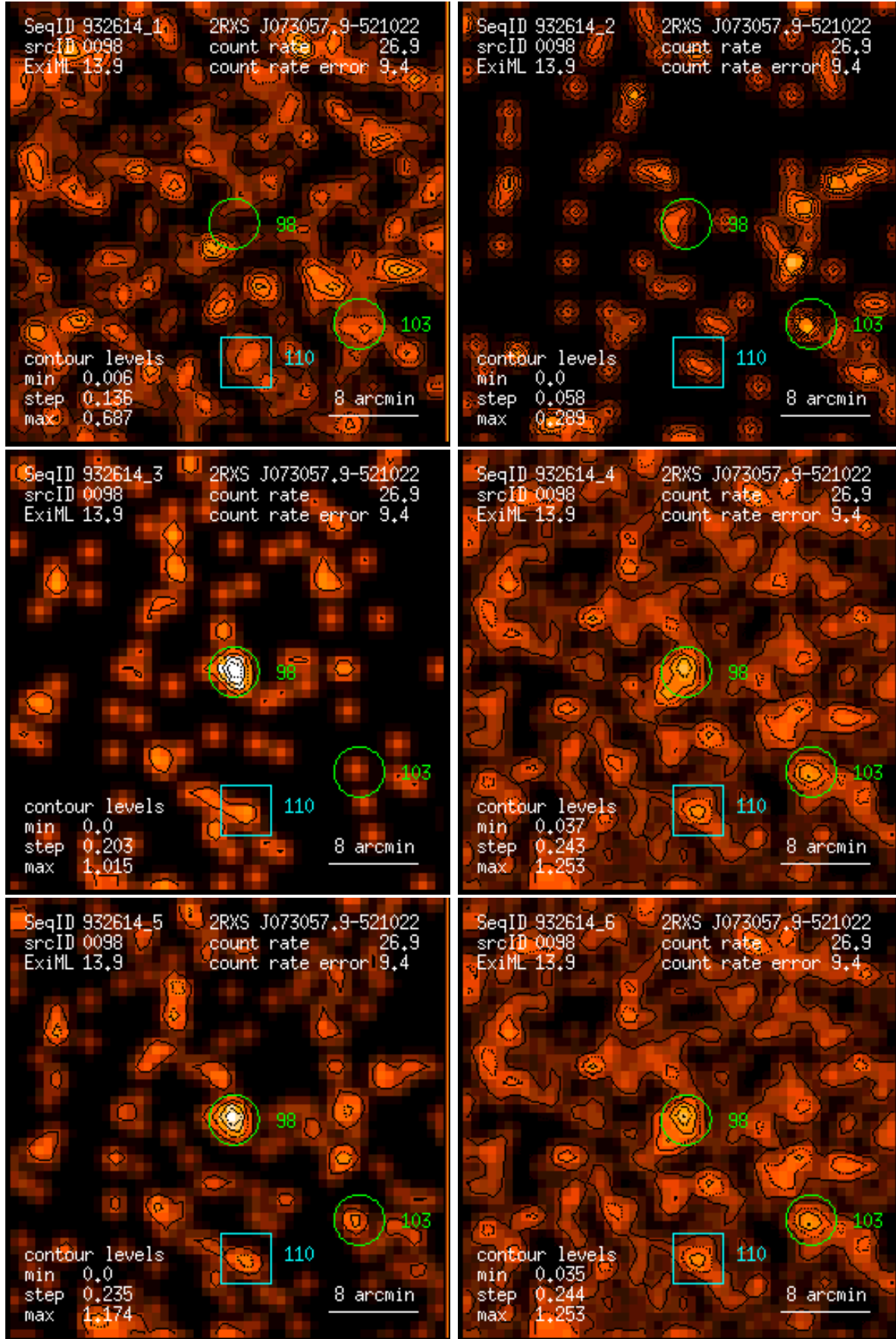
Figure 98: RASS 932614: detection 0098: band rate images, Gaussian filter: (1) PSPC channels 11 – 41, (2) 52 – 90, (3) 91 – 201, (4) 11 – 235, (5) 52 – 201, (6) 11 – 201. Broad band rates in counts/ks. Band rate contour levels in counts/ks/arcmin 2 .
