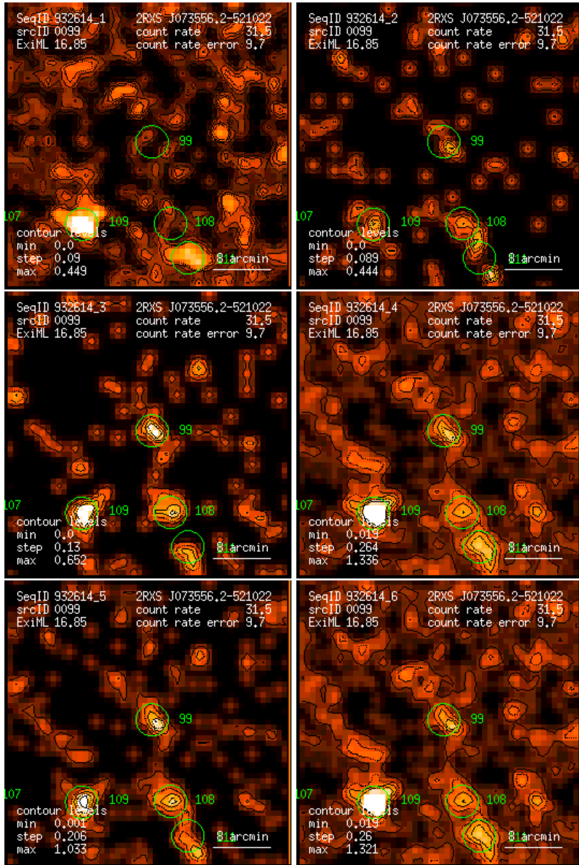
Figure 99: RASS 932614: detection 0099: band rate images, Gaussian filter: (1) PSPC channels 11 – 41, (2) 52 – 90, (3) 91 – 201, (4) 11 – 235, (5) 52 – 201, (6) 11 – 201. Broad band rates in counts/ks. Band rate contour levels in counts/ks/arcmin 2 .
