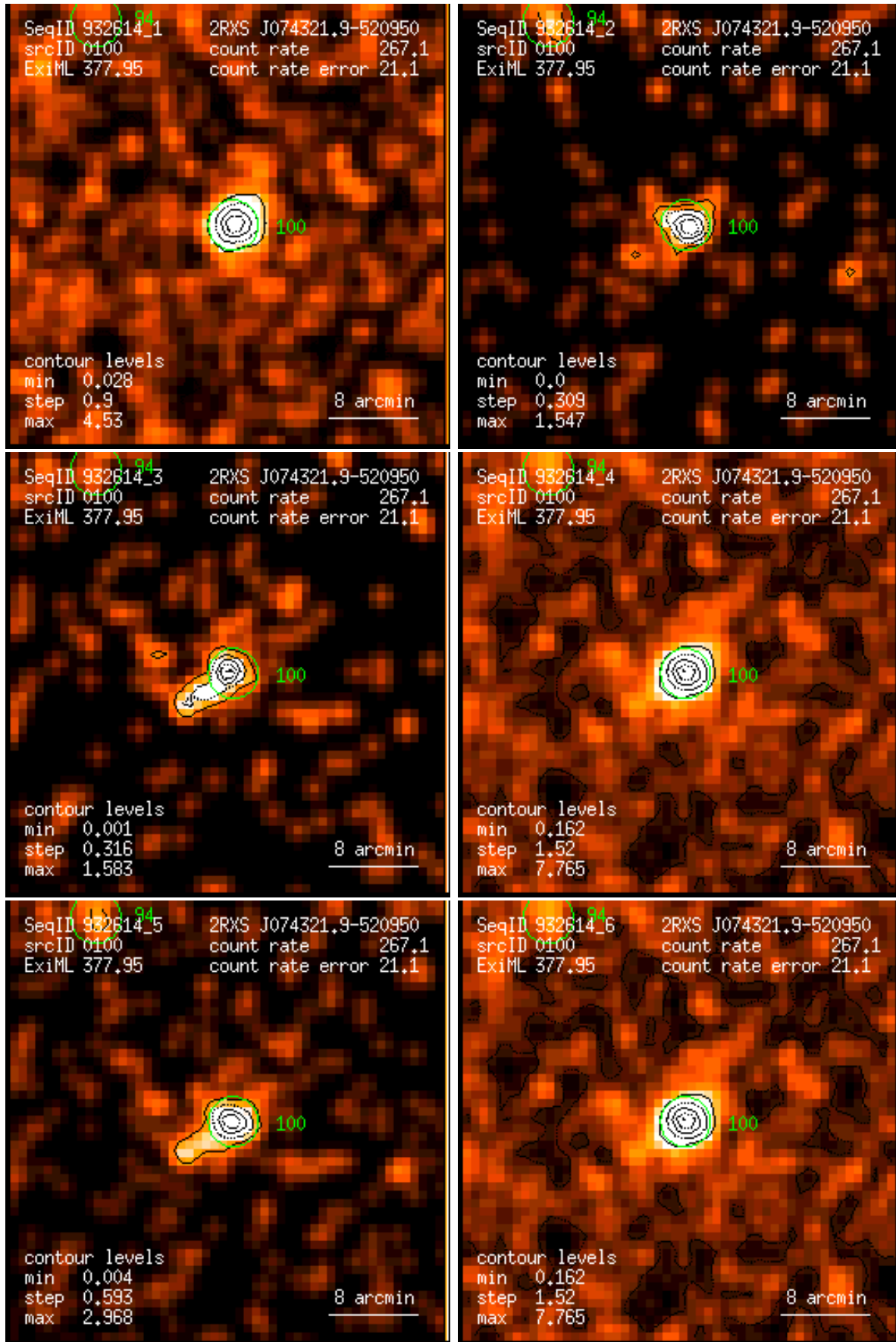
Figure 100: RASS 932614: detection 0100: band rate images, Gaussian filter: (1) PSPC channels 11 – 41, (2) 52 – 90, (3) 91 – 201, (4) 11 – 235, (5) 52 – 201, (6) 11 – 201. Broad band rates in counts/ks. Band rate contour levels in counts/ks/arcmin 2 .
