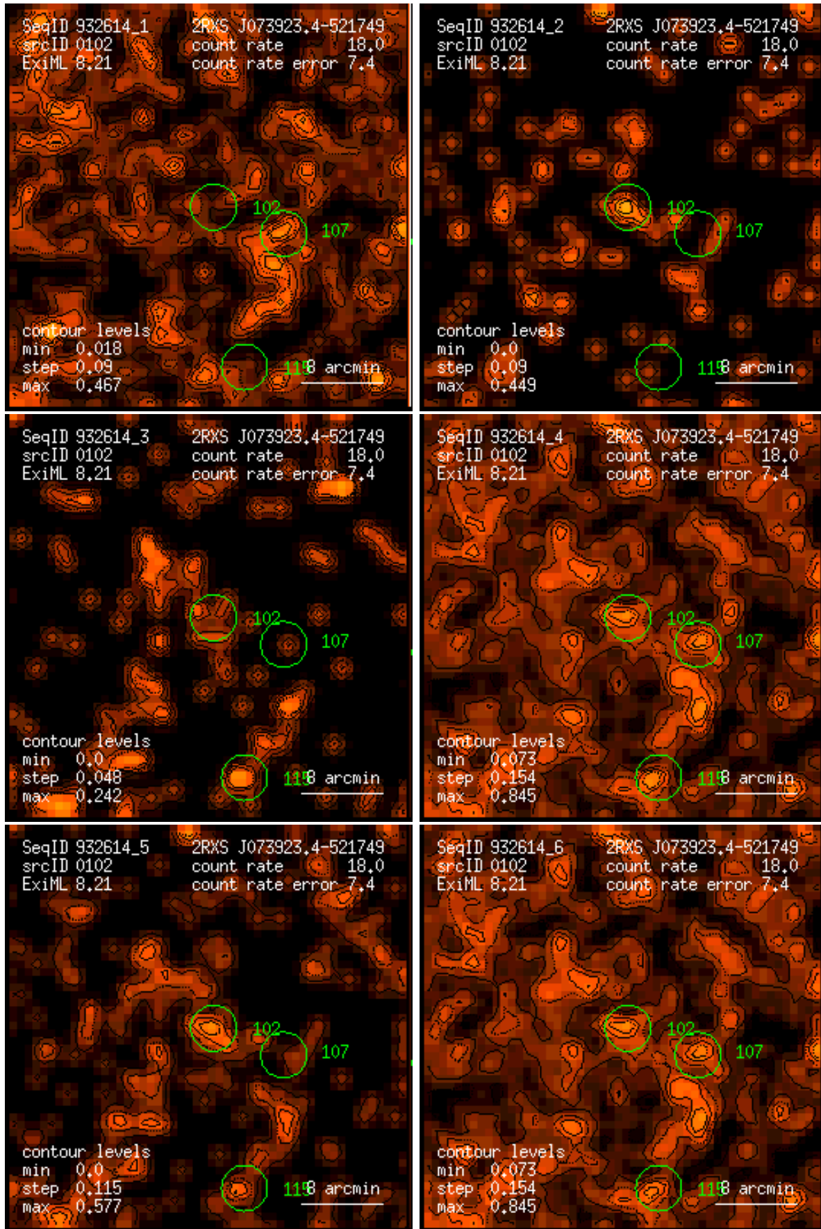
Figure 102: RASS 932614: detection 0102: band rate images, Gaussian filter: (1) PSPC channels 11 – 41, (2) 52 – 90, (3) 91 – 201, (4) 11 – 235, (5) 52 – 201, (6) 11 – 201. Broad band rates in counts/ks. Band rate contour levels in counts/ks/arcmin 2 .
