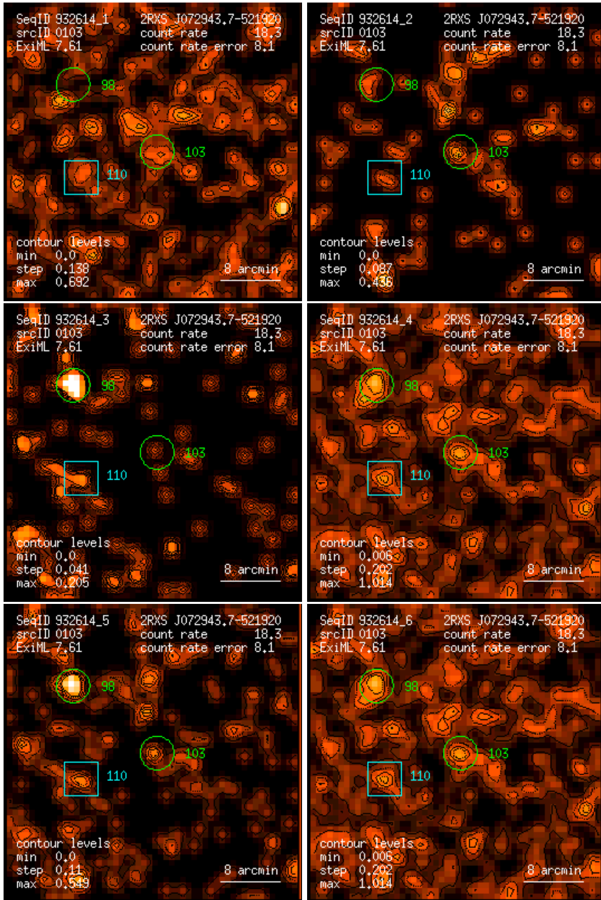
Figure 103: RASS 932614: detection 0103: band rate images, Gaussian filter: (1) PSPC channels 11 – 41, (2) 52 – 90, (3) 91 – 201, (4) 11 – 235, (5) 52 – 201, (6) 11 – 201. Broad band rates in counts/ks. Band rate contour levels in counts/ks/arcmin 2 .
