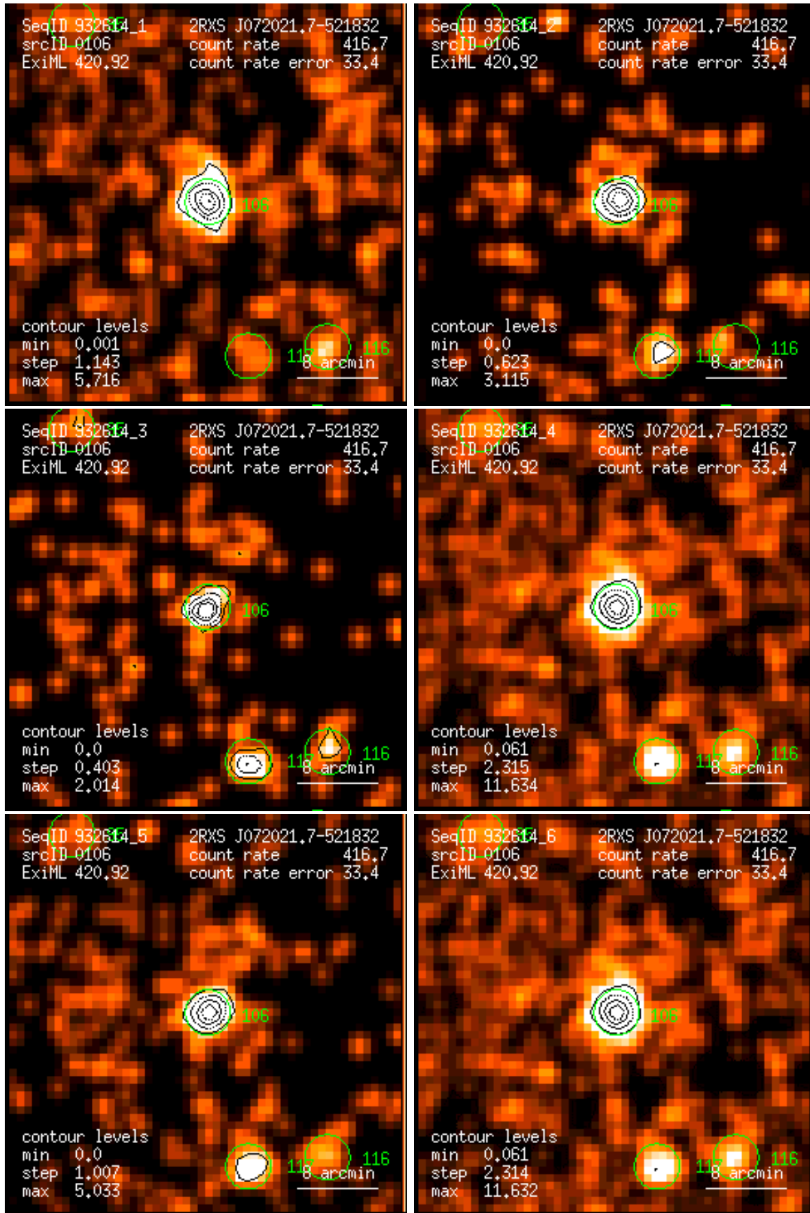
Figure 106: RASS 932614: detection 0106: band rate images, Gaussian filter: (1) PSPC channels 11 – 41, (2) 52 – 90, (3) 91 – 201, (4) 11 – 235, (5) 52 – 201, (6) 11 – 201. Broad band rates in counts/ks. Band rate contour levels in counts/ks/arcmin 2 .
