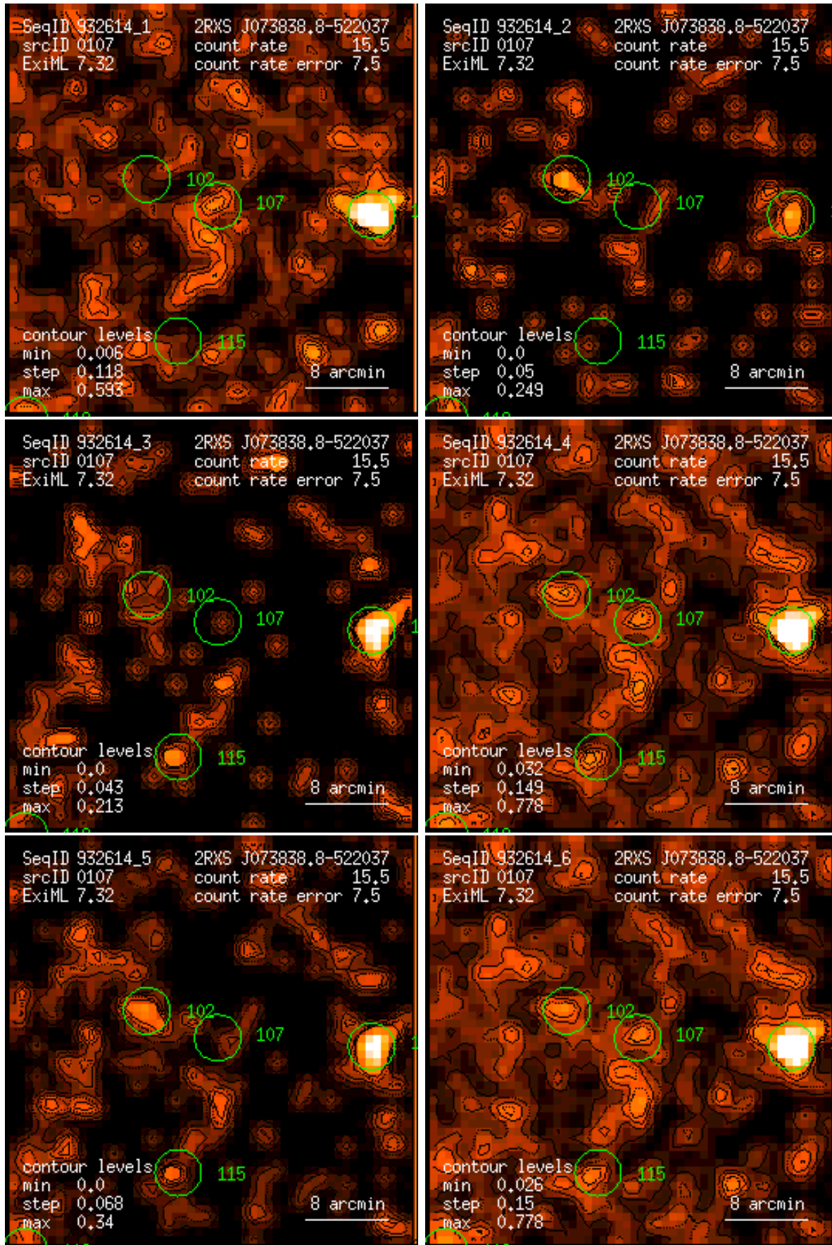
Figure 107: RASS 932614: detection 0107: band rate images, Gaussian filter: (1) PSPC channels 11 – 41, (2) 52 – 90, (3) 91 – 201, (4) 11 – 235, (5) 52 – 201, (6) 11 – 201. Broad band rates in counts/ks. Band rate contour levels in counts/ks/arcmin 2 .
