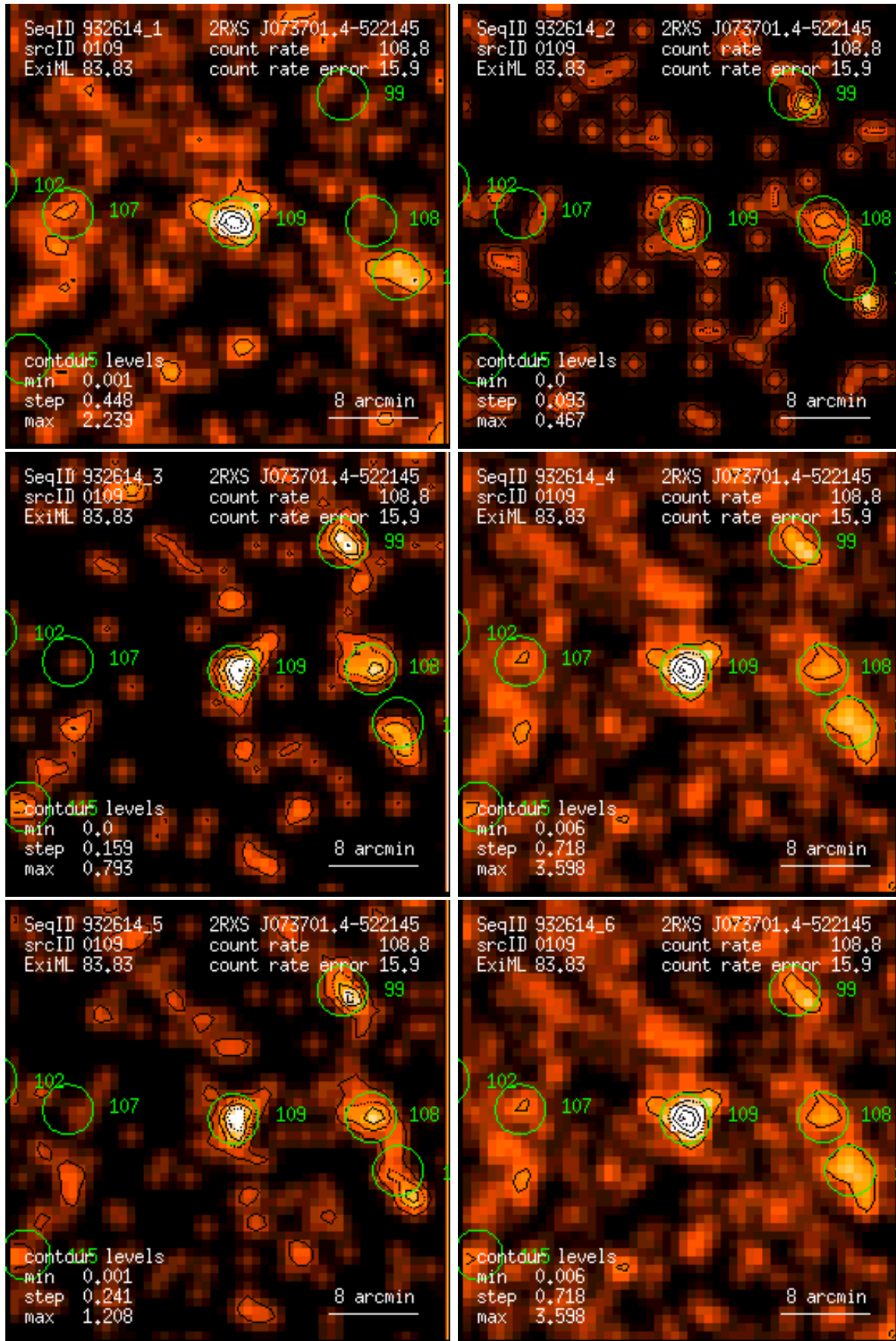
Figure 109: RASS 932614: detection 0109: band rate images, Gaussian filter: (1) PSPC channels 11 – 41, (2) 52 – 90, (3) 91 – 201, (4) 11 – 235, (5) 52 – 201, (6) 11 – 201. Broad band rates in counts/ks. Band rate contour levels in counts/ks/arcmin 2 .
