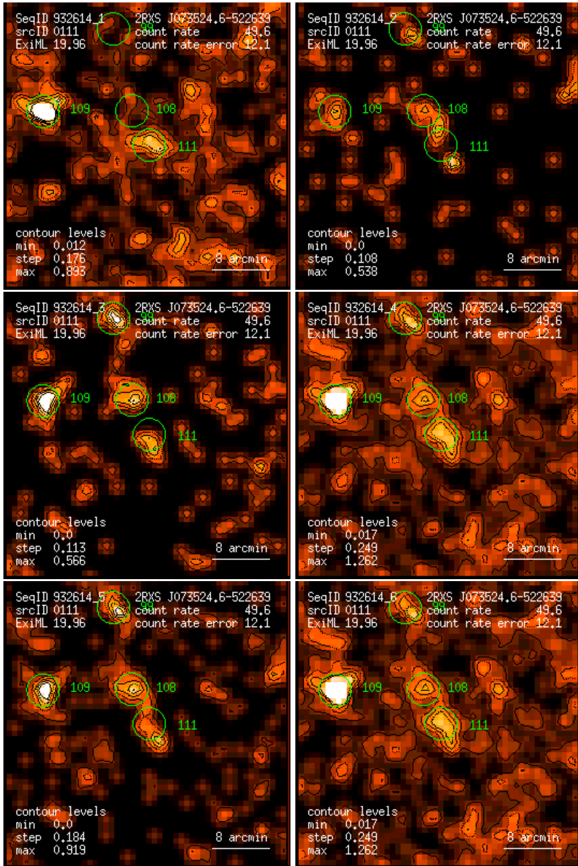
Figure 111: RASS 932614: detection 0111: band rate images, Gaussian filter: (1) PSPC channels 11 – 41, (2) 52 – 90, (3) 91 – 201, (4) 11 – 235, (5) 52 – 201, (6) 11 – 201. Broad band rates in counts/ks. Band rate contour levels in counts/ks/arcmin 2 .
