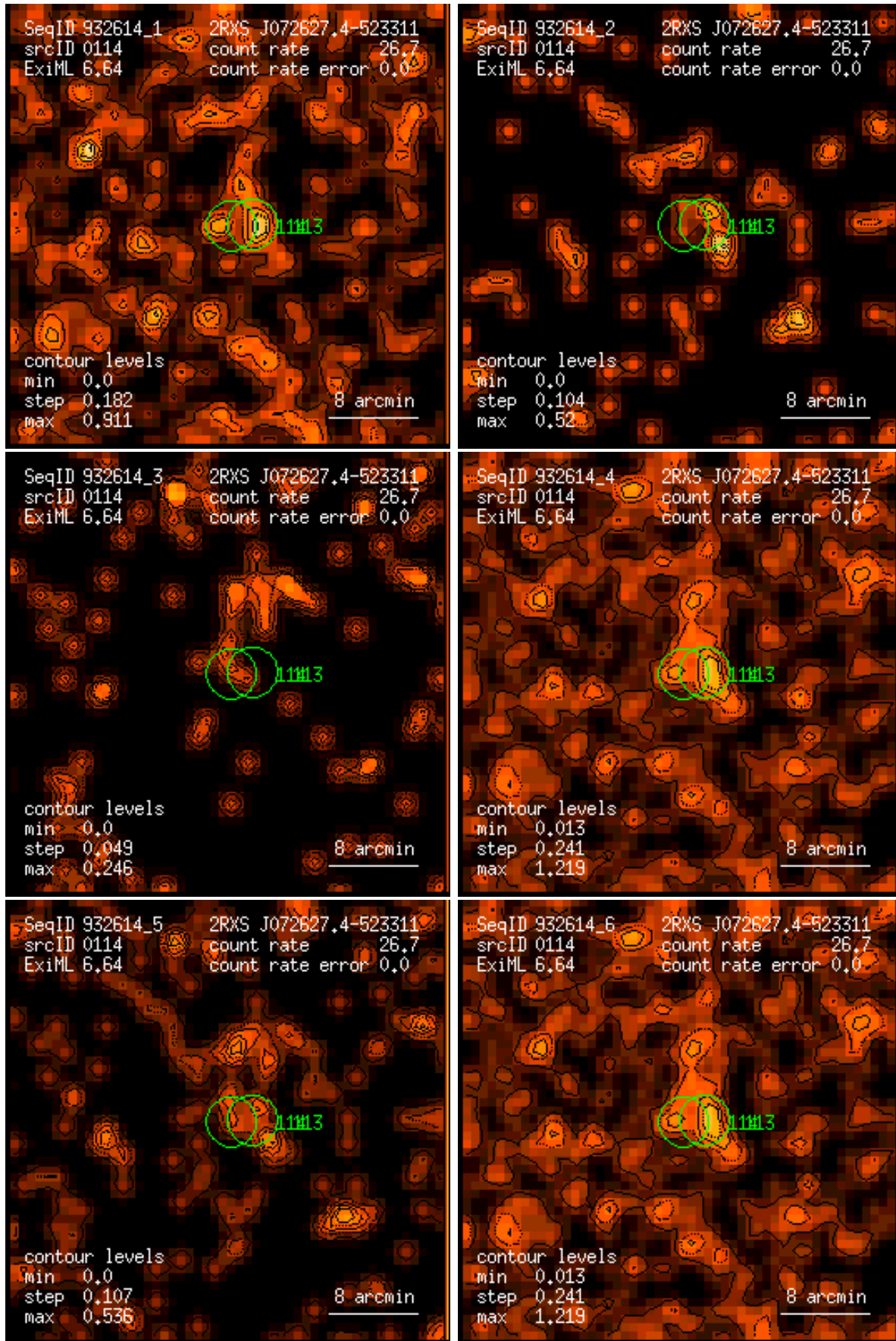
Figure 114: RASS 932614: detection 0114: band rate images, Gaussian filter: (1) PSPC channels 11 – 41, (2) 52 – 90, (3) 91 – 201, (4) 11 – 235, (5) 52 – 201, (6) 11 – 201. Broad band rates in counts/ks. Band rate contour levels in counts/ks/arcmin 2 .
