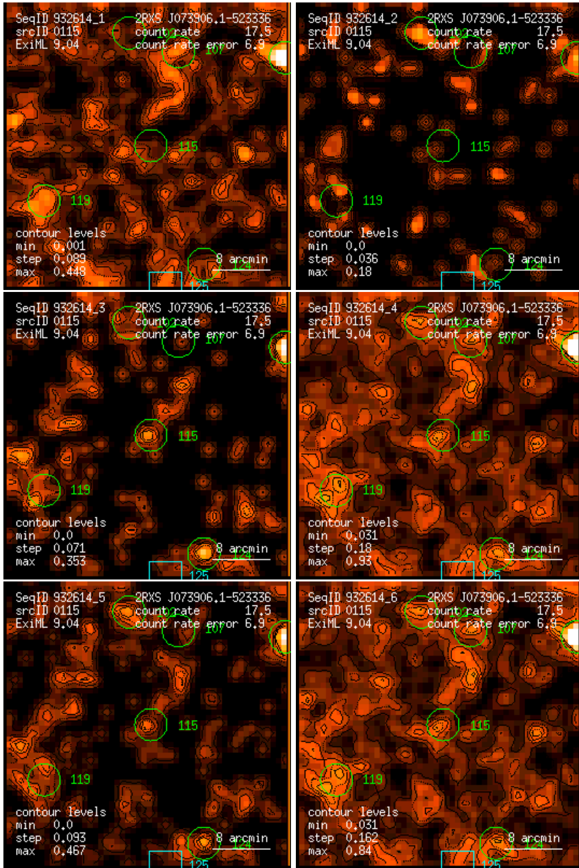
Figure 115: RASS 932614: detection 0115: band rate images, Gaussian filter: (1) PSPC channels 11 – 41, (2) 52 – 90, (3) 91 – 201, (4) 11 – 235, (5) 52 – 201, (6) 11 – 201. Broad band rates in counts/ks. Band rate contour levels in counts/ks/arcmin 2 .
