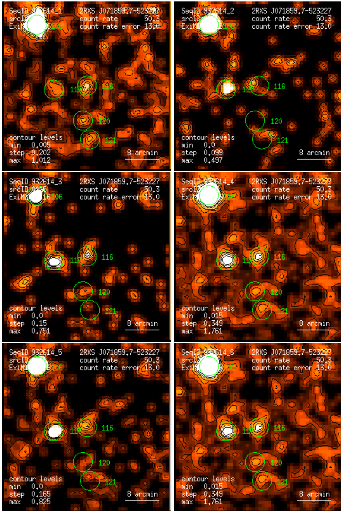
Figure 116: RASS 932614: detection 0116: band rate images, Gaussian filter: (1) PSPC channels 11 – 41, (2) 52 – 90, (3) 91 – 201, (4) 11 – 235, (5) 52 – 201, (6) 11 – 201. Broad band rates in counts/ks. Band rate contour levels in counts/ks/arcmin 2 .
