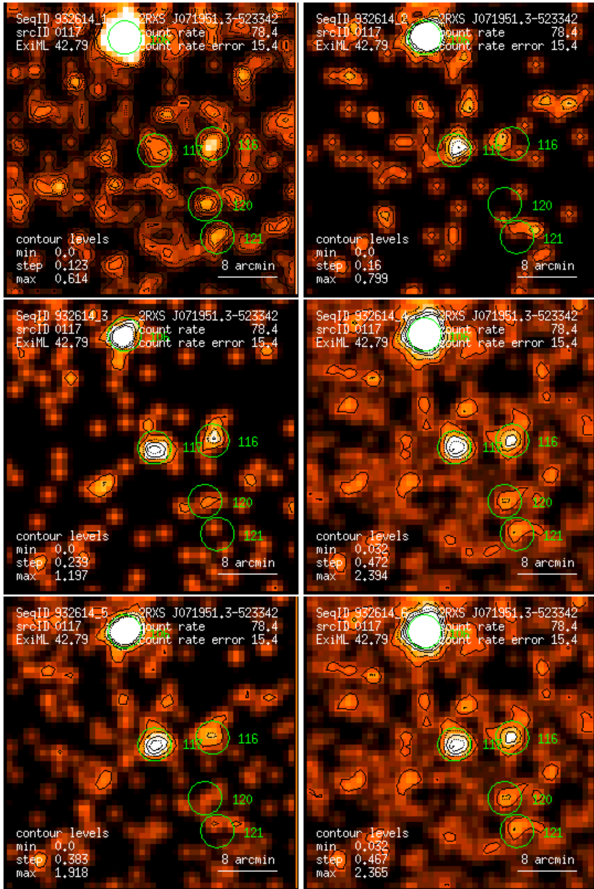
Figure 117: RASS 932614: detection 0117: band rate images, Gaussian filter: (1) PSPC channels 11 – 41, (2) 52 – 90, (3) 91 – 201, (4) 11 – 235, (5) 52 – 201, (6) 11 – 201. Broad band rates in counts/ks. Band rate contour levels in counts/ks/arcmin 2 .
