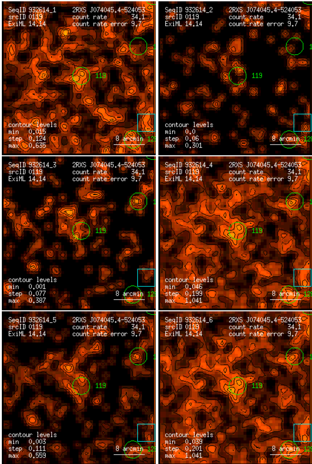
Figure 119: RASS 932614: detection 0119: band rate images, Gaussian filter: (1) PSPC channels 11 – 41, (2) 52 – 90, (3) 91 – 201, (4) 11 – 235, (5) 52 – 201, (6) 11 – 201. Broad band rates in counts/ks. Band rate contour levels in counts/ks/arcmin 2 .
