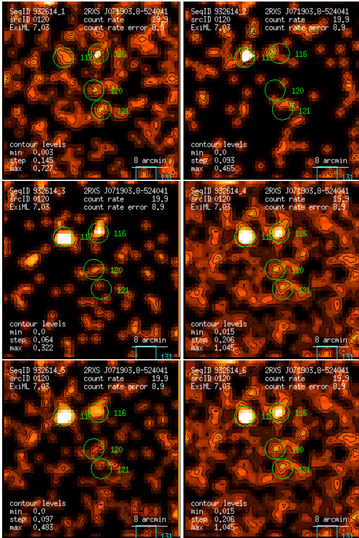
Figure 120: RASS 932614: detection 0120: band rate images, Gaussian filter: (1) PSPC channels 11 – 41, (2) 52 – 90, (3) 91 – 201, (4) 11 – 235, (5) 52 – 201, (6) 11 – 201. Broad band rates in counts/ks. Band rate contour levels in counts/ks/arcmin 2 .
