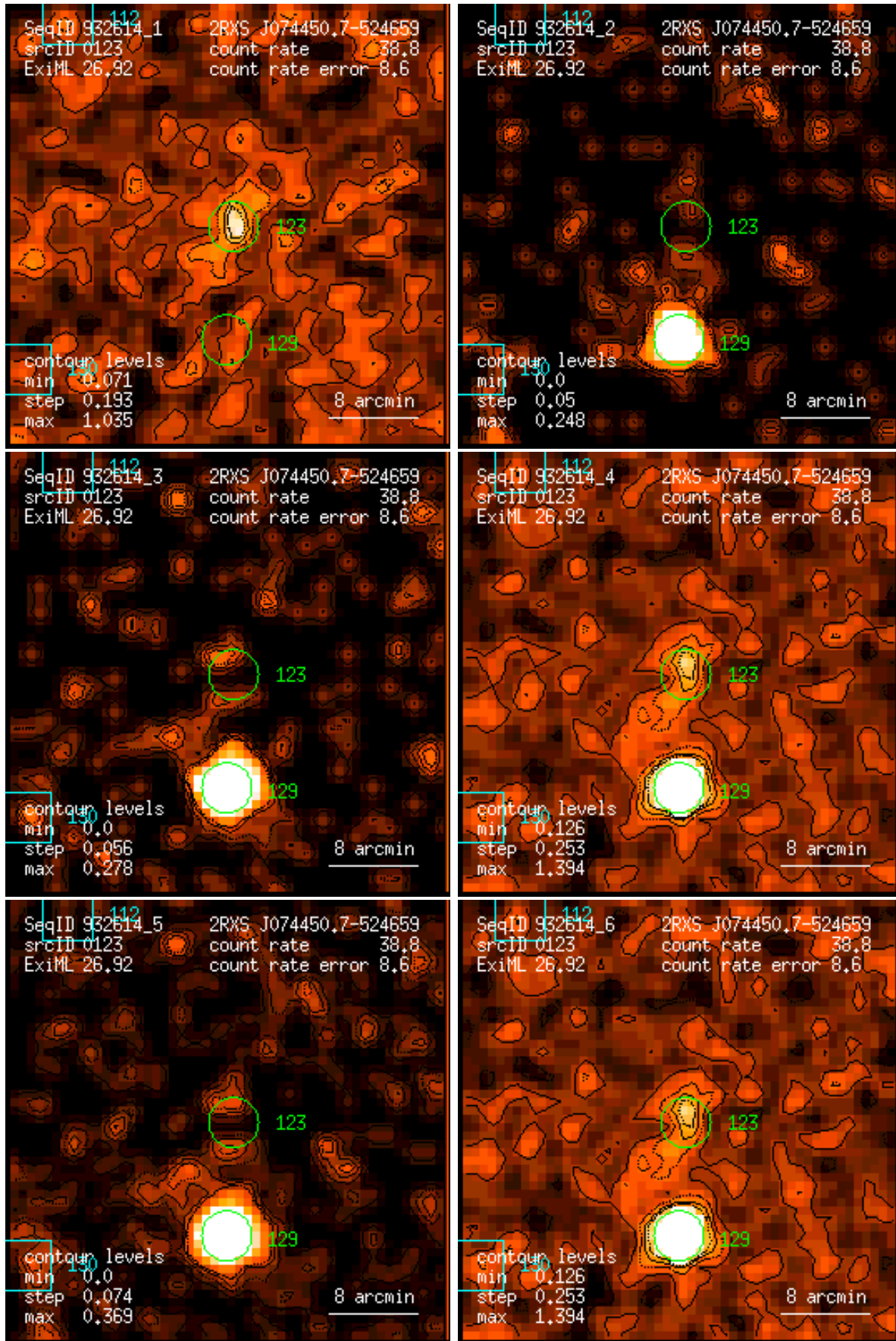
Figure 123: RASS 932614: detection 0123: band rate images, Gaussian filter: (1) PSPC channels 11 – 41, (2) 52 – 90, (3) 91 – 201, (4) 11 – 235, (5) 52 – 201, (6) 11 – 201. Broad band rates in counts/ks. Band rate contour levels in counts/ks/arcmin 2 .
