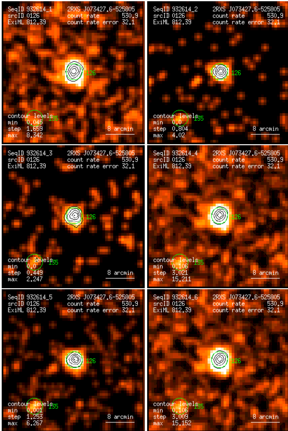
Figure 126: RASS 932614: detection 0126: band rate images, Gaussian filter: (1) PSPC channels 11 – 41, (2) 52 – 90, (3) 91 – 201, (4) 11 – 235, (5) 52 – 201, (6) 11 – 201. Broad band rates in counts/ks. Band rate contour levels in counts/ks/arcmin 2 .
