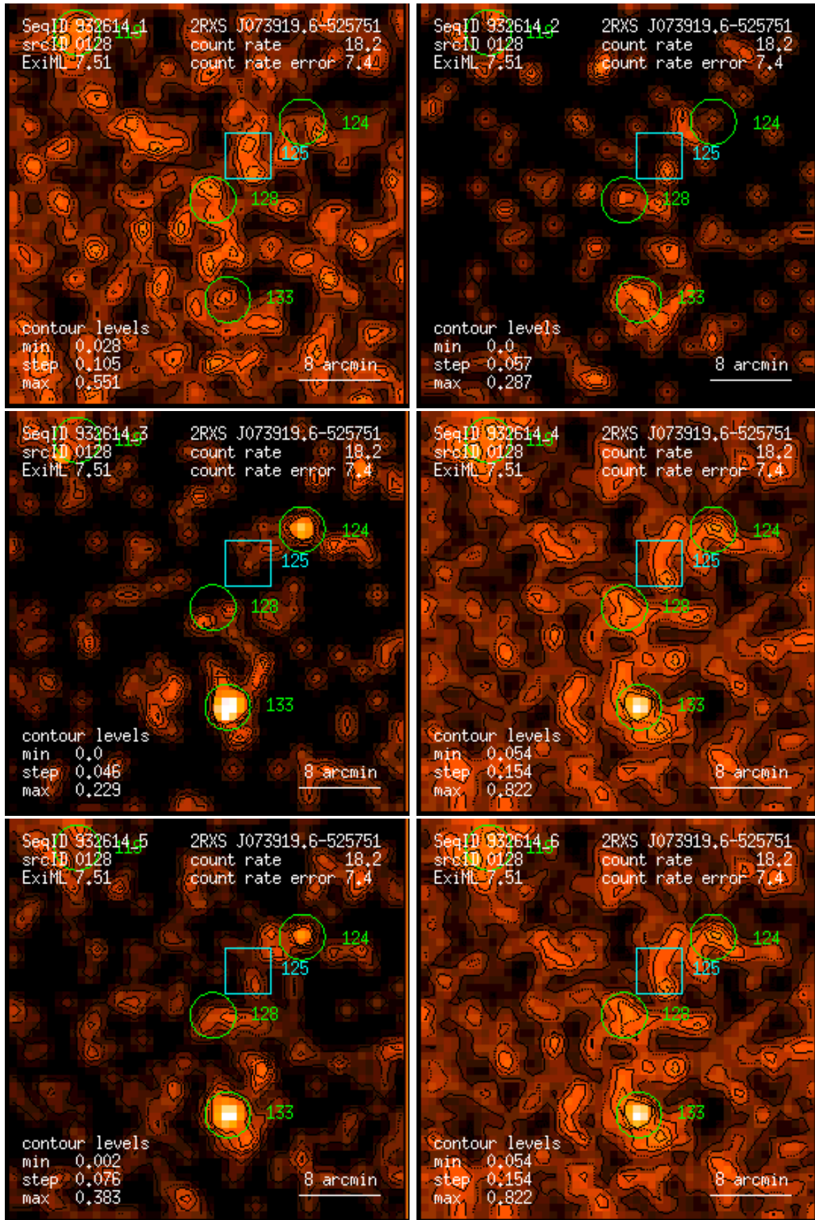
Figure 128: RASS 932614: detection 0128: band rate images, Gaussian filter: (1) PSPC channels 11 – 41, (2) 52 – 90, (3) 91 – 201, (4) 11 – 235, (5) 52 – 201, (6) 11 – 201. Broad band rates in counts/ks. Band rate contour levels in counts/ks/arcmin 2 .
