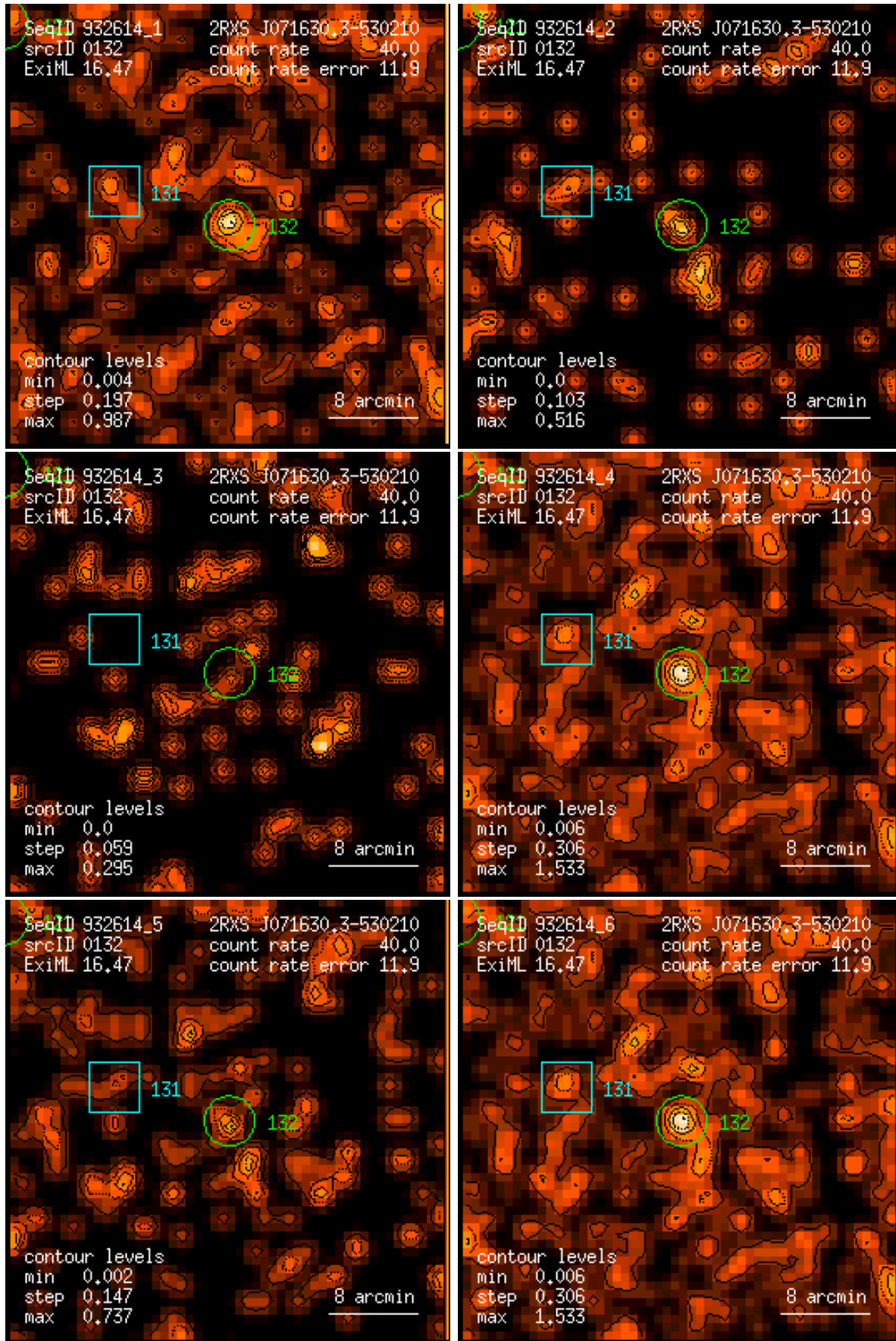
Figure 132: RASS 932614: detection 0132: band rate images, Gaussian filter: (1) PSPC channels 11 – 41, (2) 52 – 90, (3) 91 – 201, (4) 11 – 235, (5) 52 – 201, (6) 11 – 201. Broad band rates in counts/ks. Band rate contour levels in counts/ks/arcmin 2 .
