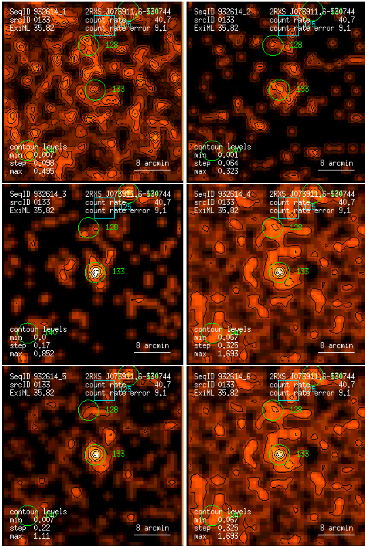
Figure 133: RASS 932614: detection 0133: band rate images, Gaussian filter: (1) PSPC channels 11 – 41, (2) 52 – 90, (3) 91 – 201, (4) 11 – 235, (5) 52 – 201, (6) 11 – 201. Broad band rates in counts/ks. Band rate contour levels in counts/ks/arcmin 2 .
