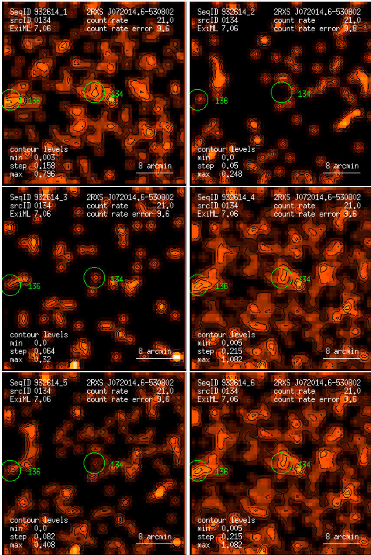
Figure 134: RASS 932614: detection 0134: band rate images, Gaussian filter: (1) PSPC channels 11 – 41, (2) 52 – 90, (3) 91 – 201, (4) 11 – 235, (5) 52 – 201, (6) 11 – 201. Broad band rates in counts/ks. Band rate contour levels in counts/ks/arcmin 2 .
