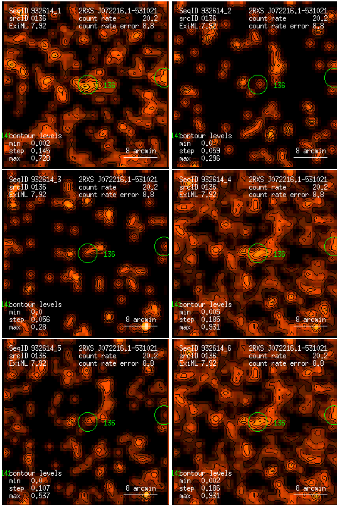
Figure 136: RASS 932614: detection 0136: band rate images, Gaussian filter: (1) PSPC channels 11 – 41, (2) 52 – 90, (3) 91 – 201, (4) 11 – 235, (5) 52 – 201, (6) 11 – 201. Broad band rates in counts/ks. Band rate contour levels in counts/ks/arcmin 2 .
