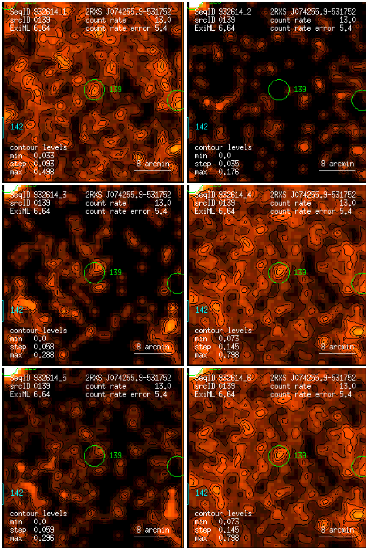
Figure 139: RASS 932614: detection 0139: band rate images, Gaussian filter: (1) PSPC channels 11 – 41, (2) 52 – 90, (3) 91 – 201, (4) 11 – 235, (5) 52 – 201, (6) 11 – 201. Broad band rates in counts/ks. Band rate contour levels in counts/ks/arcmin 2 .
