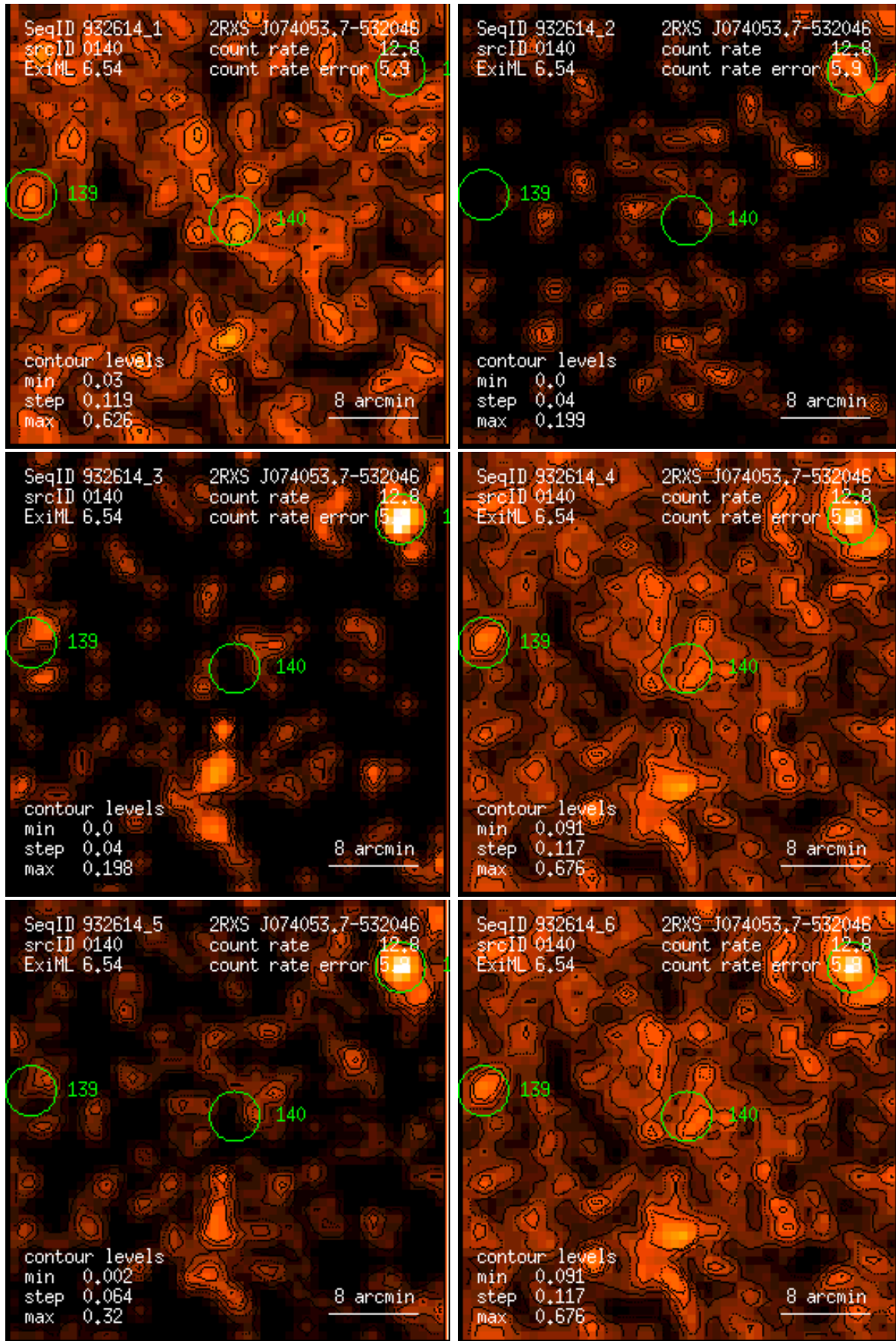
Figure 140: RASS 932614: detection 0140: band rate images, Gaussian filter: (1) PSPC channels 11 – 41, (2) 52 – 90, (3) 91 – 201, (4) 11 – 235, (5) 52 – 201, (6) 11 – 201. Broad band rates in counts/ks. Band rate contour levels in counts/ks/arcmin 2 .
