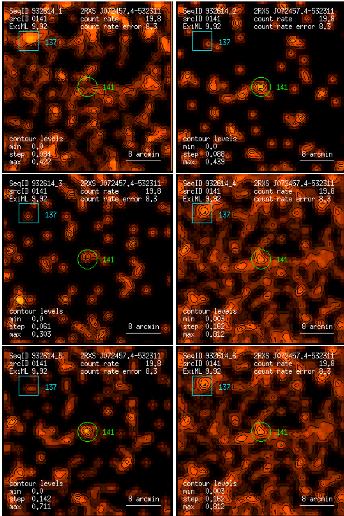
Figure 141: RASS 932614: detection 0141: band rate images, Gaussian filter: (1) PSPC channels 11 – 41, (2) 52 – 90, (3) 91 – 201, (4) 11 – 235, (5) 52 – 201, (6) 11 – 201. Broad band rates in counts/ks. Band rate contour levels in counts/ks/arcmin 2 .
