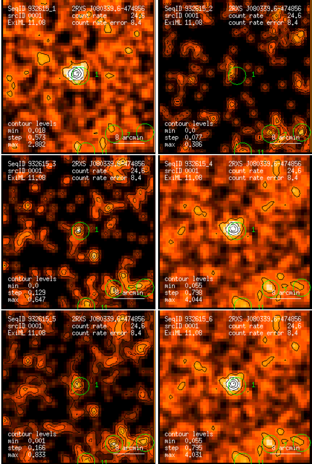
Figure 1: RASS 932615: detection 0001: band rate images, Gaussian filter: (1) PSPC channels 11 – 41, (2) 52 – 90, (3) 91 – 201, (4) 11 – 235, (5) 52 – 201, (6) 11 – 201. Broad band rates in counts/ks. Band rate contour levels in counts/ks/arcmin 2 .
