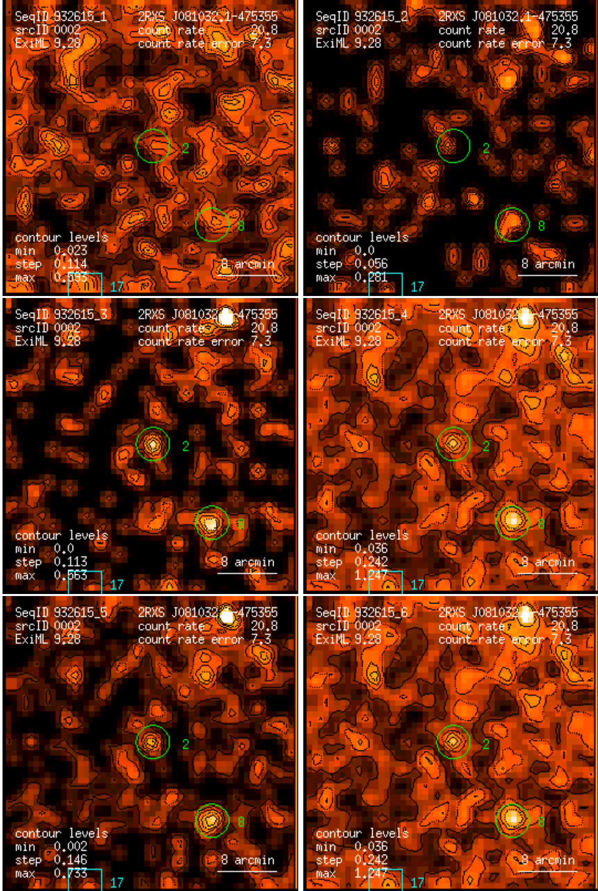
Figure 2: RASS 932615: detection 0002: band rate images, Gaussian filter: (1) PSPC channels 11 – 41, (2) 52 – 90, (3) 91 – 201, (4) 11 – 235, (5) 52 – 201, (6) 11 – 201. Broad band rates in counts/ks. Band rate contour levels in counts/ks/arcmin 2 .
