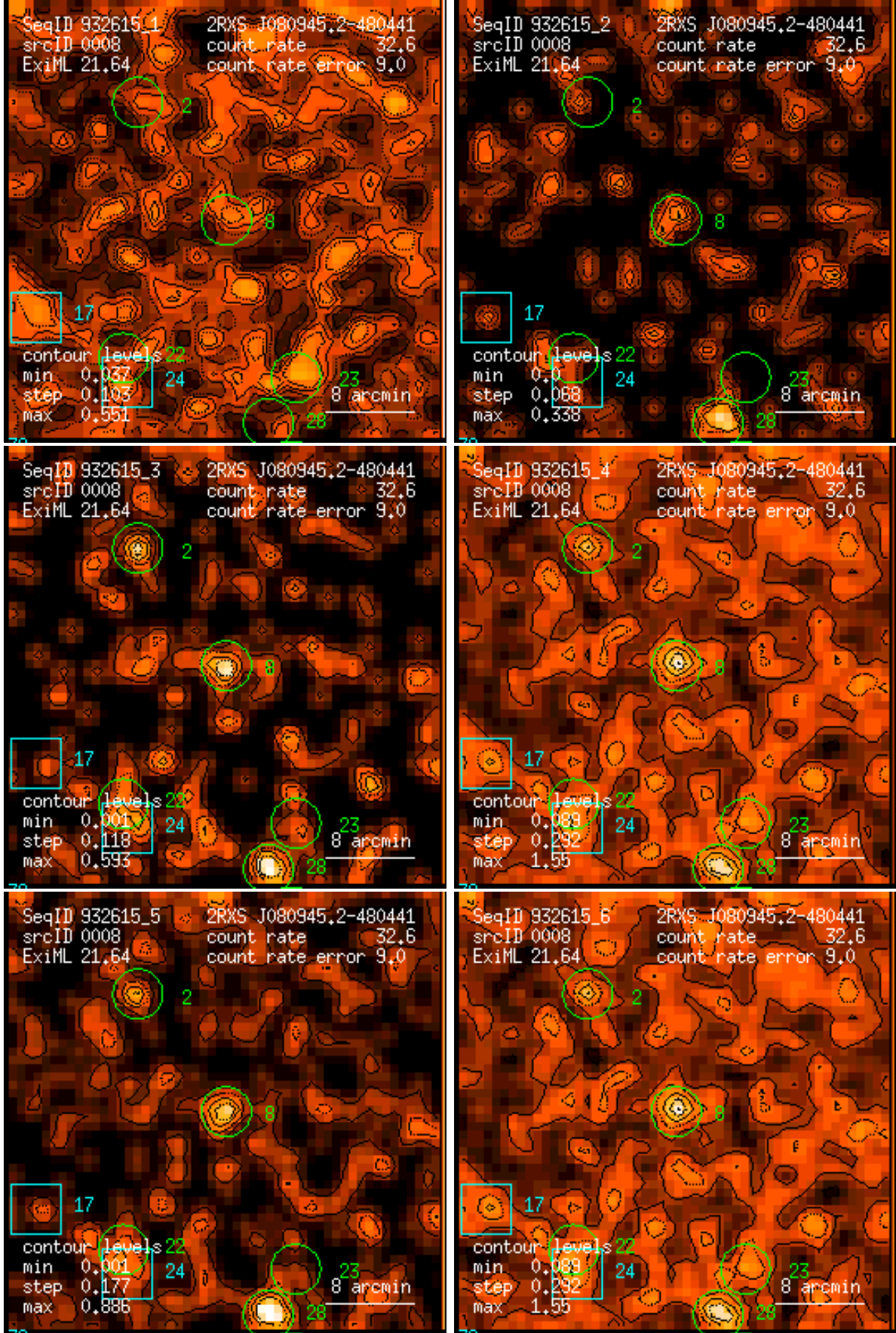
Figure 8: RASS 932615: detection 0008: band rate images, Gaussian filter: (1) PSPC channels 11 – 41, (2) 52 – 90, (3) 91 – 201, (4) 11 – 235, (5) 52 – 201, (6) 11 – 201. Broad band rates in counts/ks. Band rate contour levels in counts/ks/arcmin 2 .
