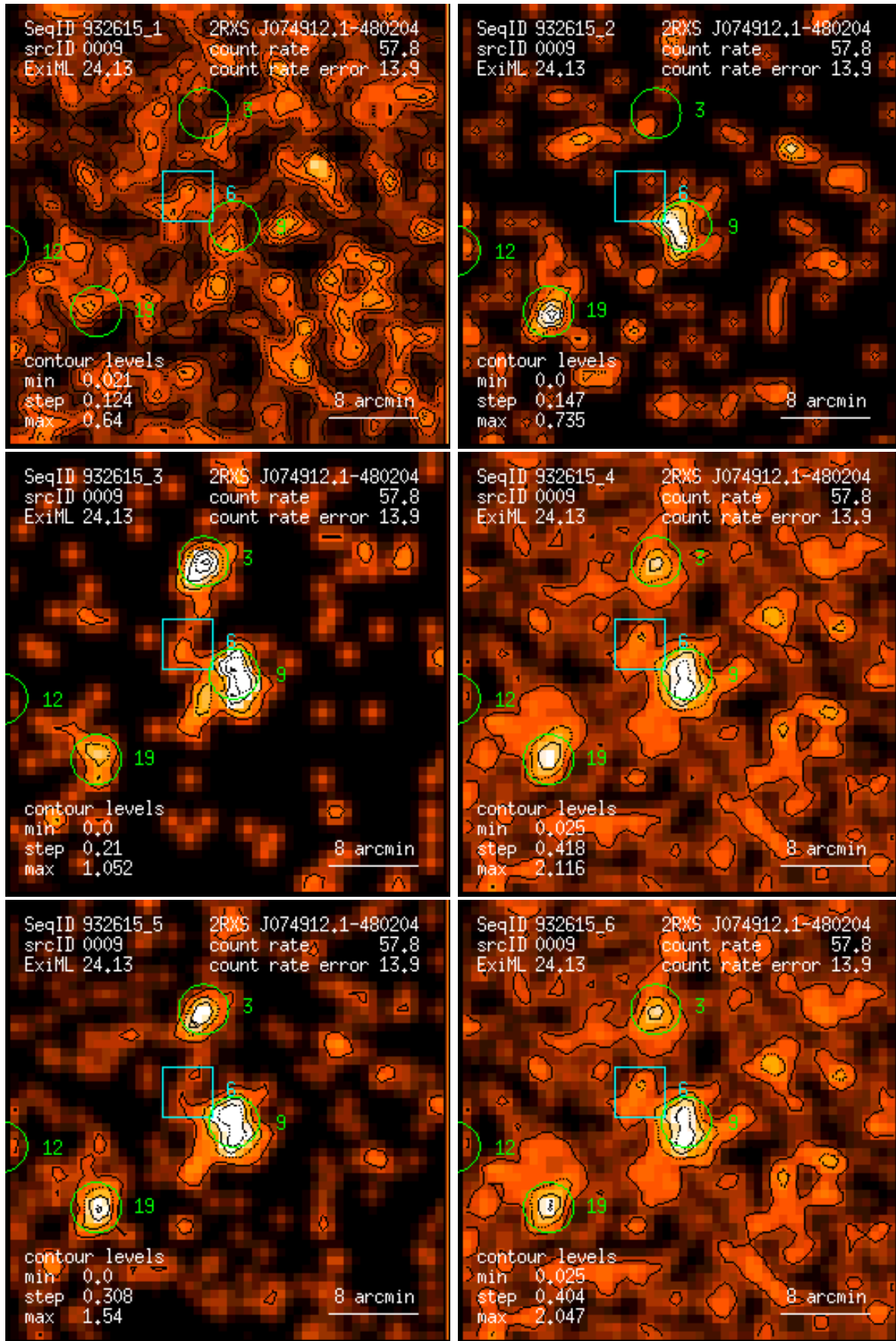
Figure 9: RASS 932615: detection 0009: band rate images, Gaussian filter: (1) PSPC channels 11 – 41, (2) 52 – 90, (3) 91 – 201, (4) 11 – 235, (5) 52 – 201, (6) 11 – 201. Broad band rates in counts/ks. Band rate contour levels in counts/ks/arcmin 2 .
