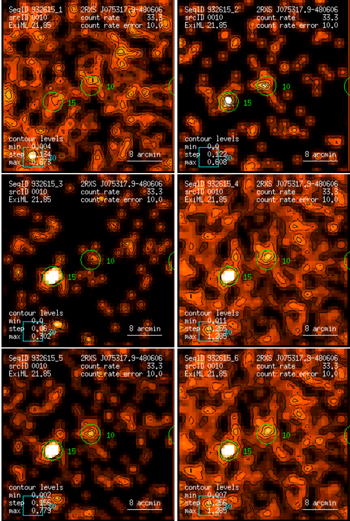
Figure 10: RASS 932615: detection 0010: band rate images, Gaussian filter: (1) PSPC channels 11 – 41, (2) 52 – 90, (3) 91 – 201, (4) 11 – 235, (5) 52 – 201, (6) 11 – 201. Broad band rates in counts/ks. Band rate contour levels in counts/ks/arcmin 2 .
